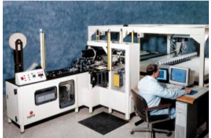
Spire's SPI-ASSEMBLER™ 5000 automated solar-cell assembler.
