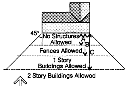
Ideal Solar Access Buildings, trees or other obstructions should not be located so as to shade the south wall of solar buildings. At this latitude, A = 17 ft., B = 30 ft., and C = 69 ft.
