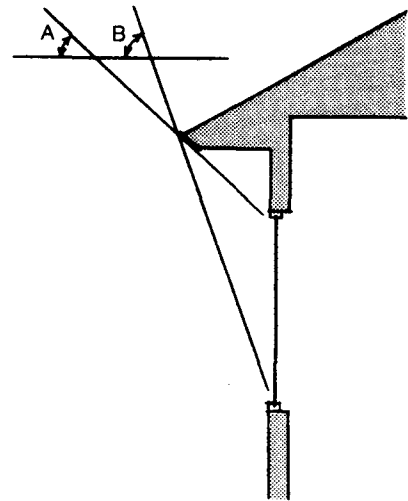
South Overhang Sizing In Farmington, an ideally sized south overhang should allow full exposure of the window when the sun has a noon altitude of 36 degrees (angle A) and fully shade the window when the sun has a noon altitude of 73 degrees (angle B).
