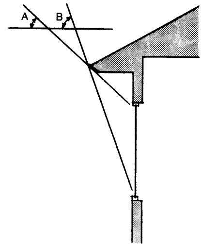
South Overhang Sizing In Salem, an ideally sized south overhang should allow full exposure of the window when the sun has a noon altitude of 26 degrees (angle A) and fully shade the window when the sun has a noon altitude of 63 degrees (angle B).
