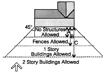
Ideal Solar Access Buildings, trees or other obstructions should not be located so as to shade the south wall of solar buildings. At this latitude, A = 8 ft., B = 13 ft., and C = 30 ft.
