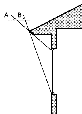
South Overhang Sizing In Charleston, an ideally sized south overhang should allow full exposure of the window when the sun has a noon altitude of 33 degrees (angle A) and fully shade the window when the sun has a noon altitude of 70 degrees (angle B).
