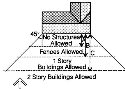
Ideal Solar Access Buildings, trees or other obstructions should not be located so as to shade the south wall of solar buildings. At this latitude, A = 12 ft., B = 21 ft., and C = 48 ft.
