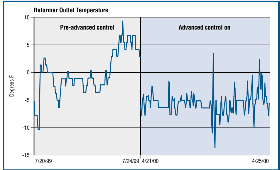
Figure 1. Primary reformer outlet temperature before and after advanced control.
