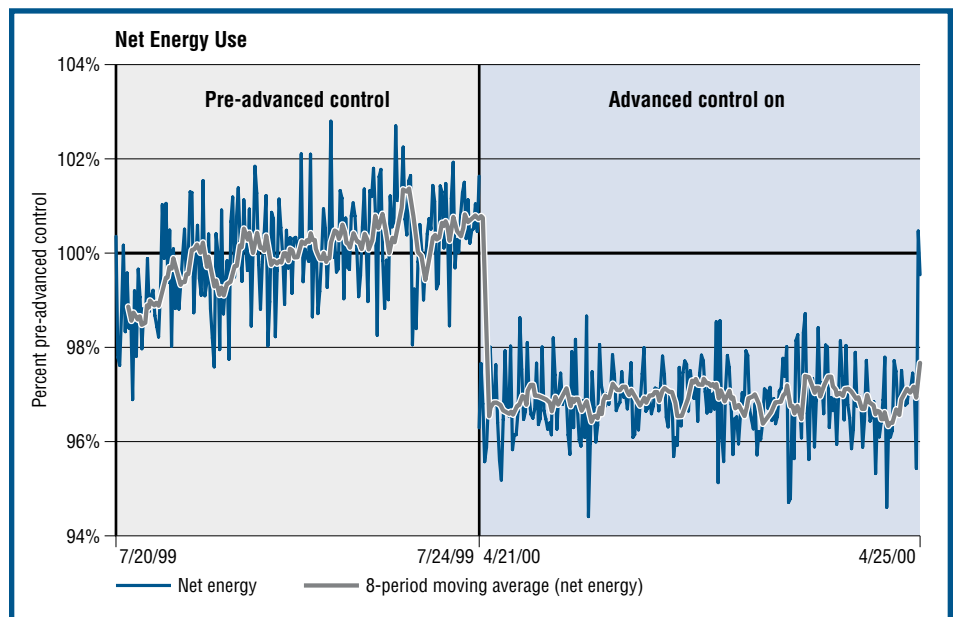
Figure 2. Net energy use in the production of methanol was reduced 2.4% after implementation of advanced process controls.
