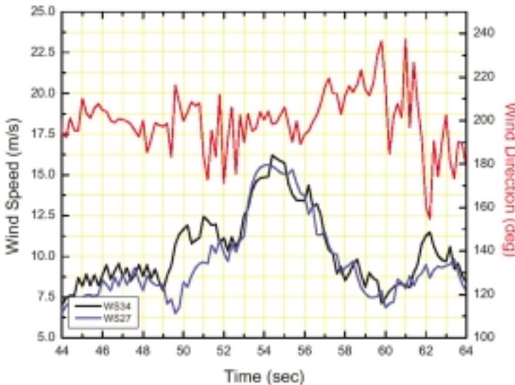
Figure 3. Wind Speed and Wind Direction Plot for Highest Recorded Rotor Speed
