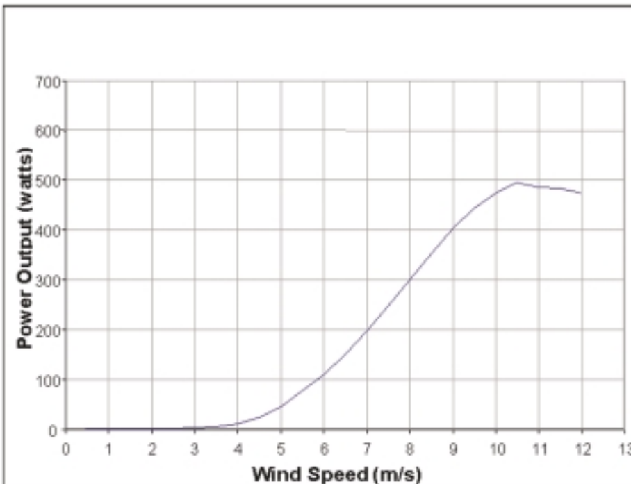
Figure 11. Whisper H40 Wind Turbine Power Curve
