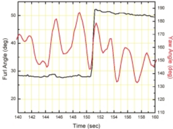
Figure 5. Furl Angle and Yaw Angle Plot for Highest Recorded Furl Rate
