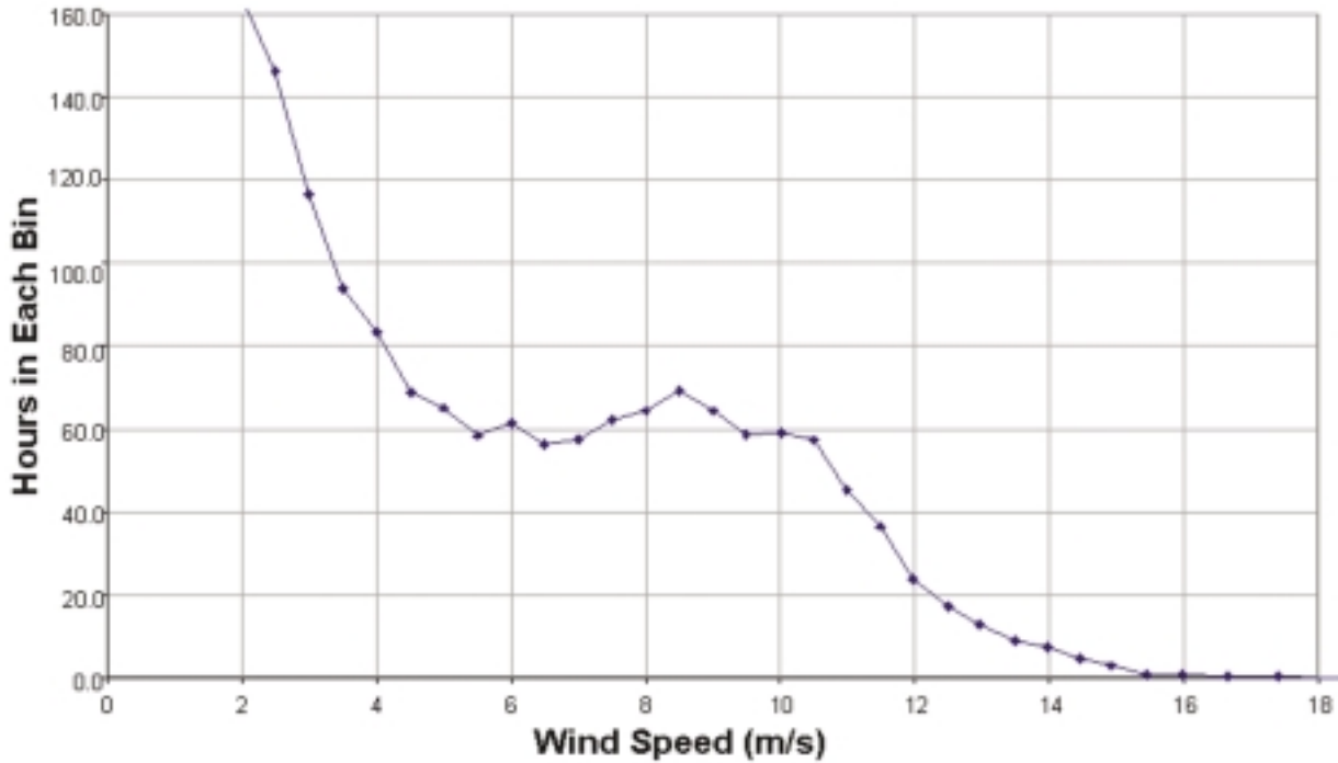
Figure 12. Wind Speed Distribution Curve
