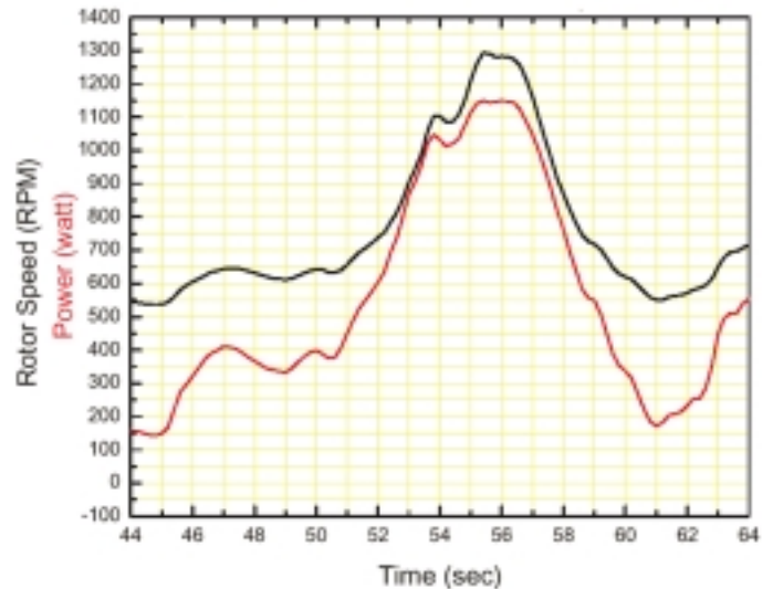
Figure 2. Rotor Speed and Power Plot for Highest Recorded Rotor Speed
