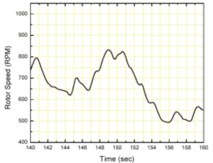
Figure 6. Rotor Speed Plot for Highest Recorded Furl Rate
