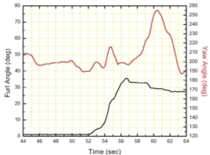
Figure 4. Furl Angle and Yaw Angle Plot for Highest Recorded Rotor Speed
