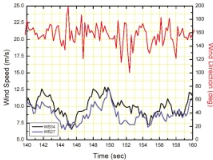
Figure 7. Wind Speed and Wind Direction Plot for Highest Recorded Furl Rate
