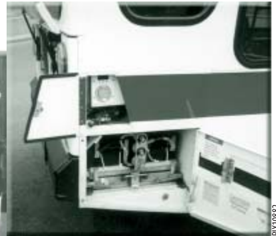
The traction battery conditioning port is above the cranking battery compartment.
