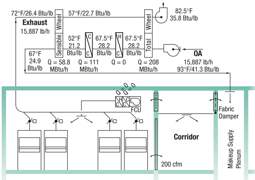
Figure 4. KINSC laboratory makeup air and comfort conditioning system. Values shown in this figure are based on the following assumptions: laboratory area of 650 ft 2 ; four VAV fume hoods, each operating at an open 900 cfm exhaust; four people working in the space, operating internal lighting and equipment load of 5 W/ft 2 ; and a summer envelope cooling load of 2400 Btu/h.
