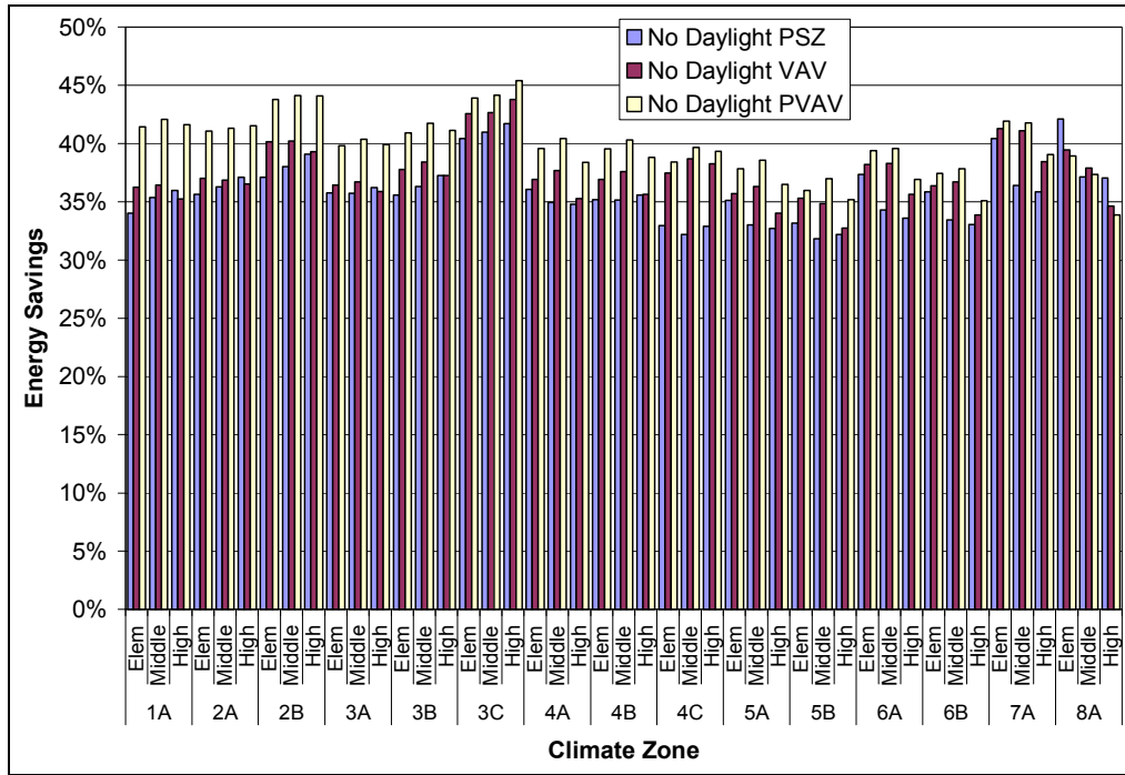
Figure 2. Energy Savings over ASHRAE 90.1-1999 for Non-daylit Schools
