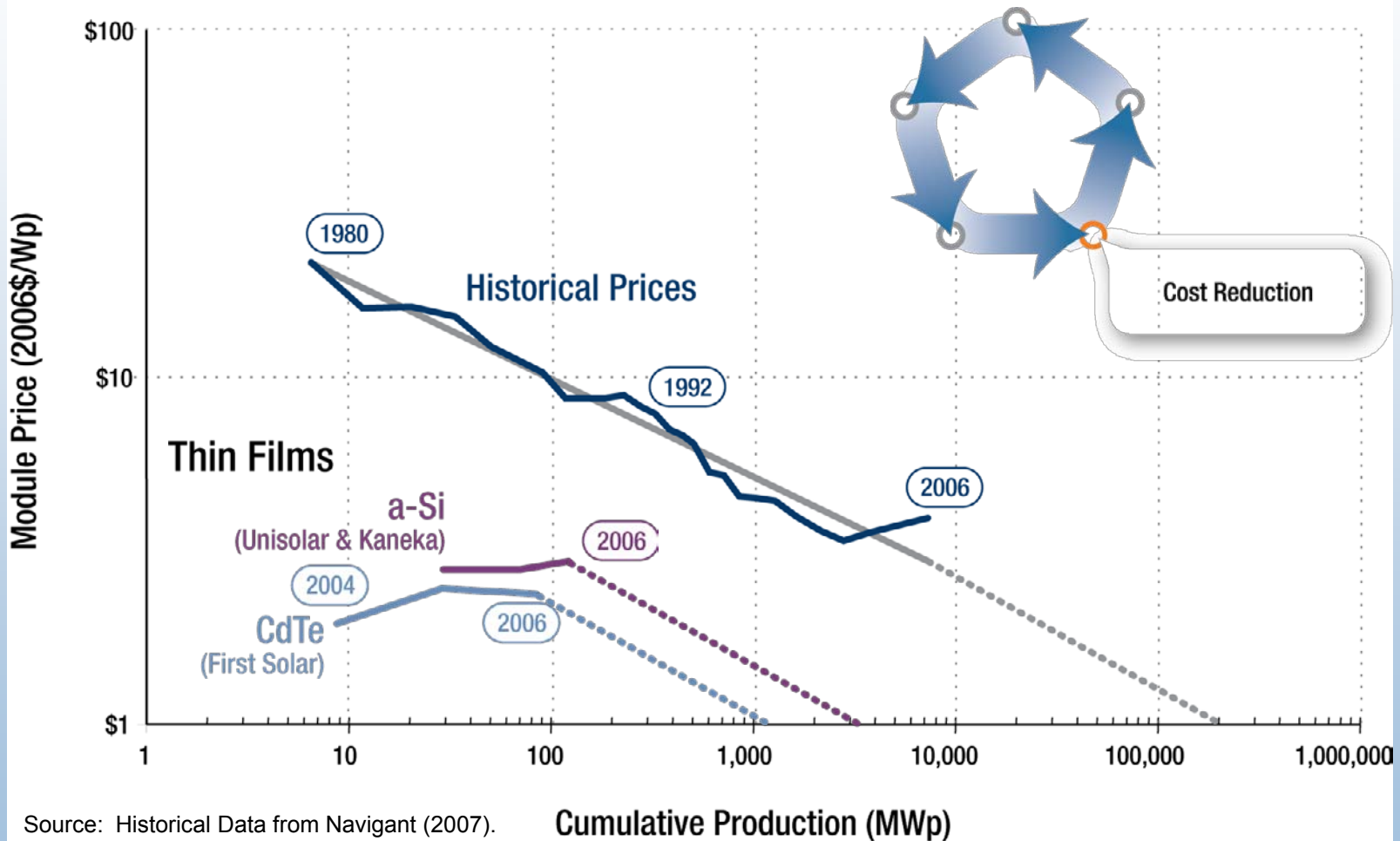
Historical and Projected Experience Curve for PV Modules
