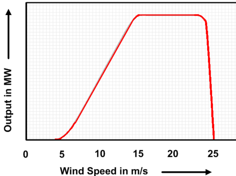
Figure 2.2. Output curve for a typical wind turbine
