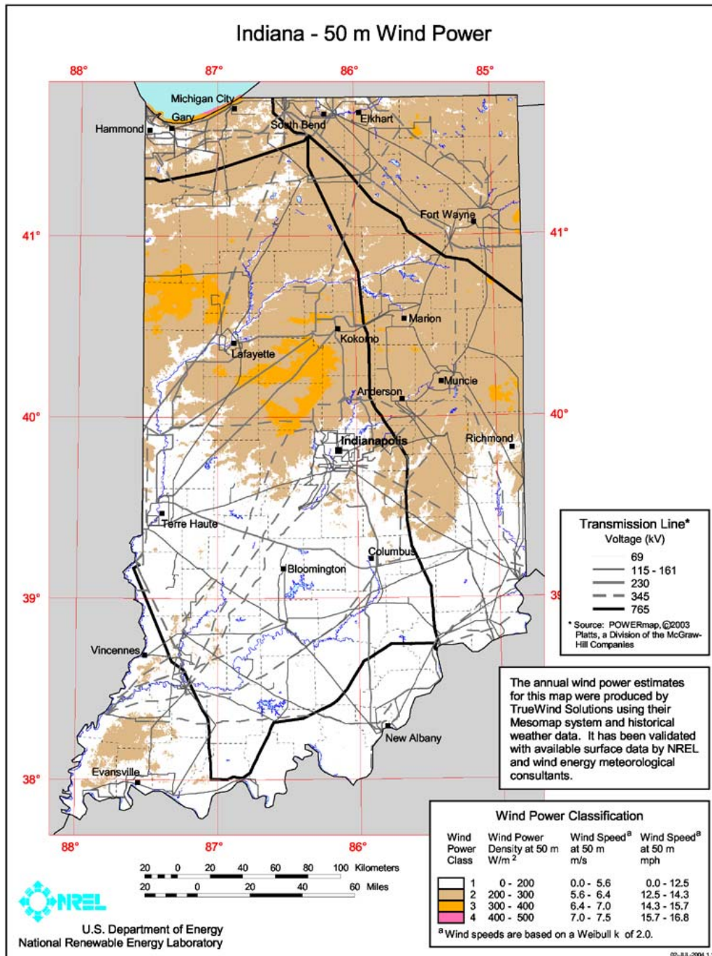
Figure 1.1.a. Indiana 50 Meter Wind Power Map
