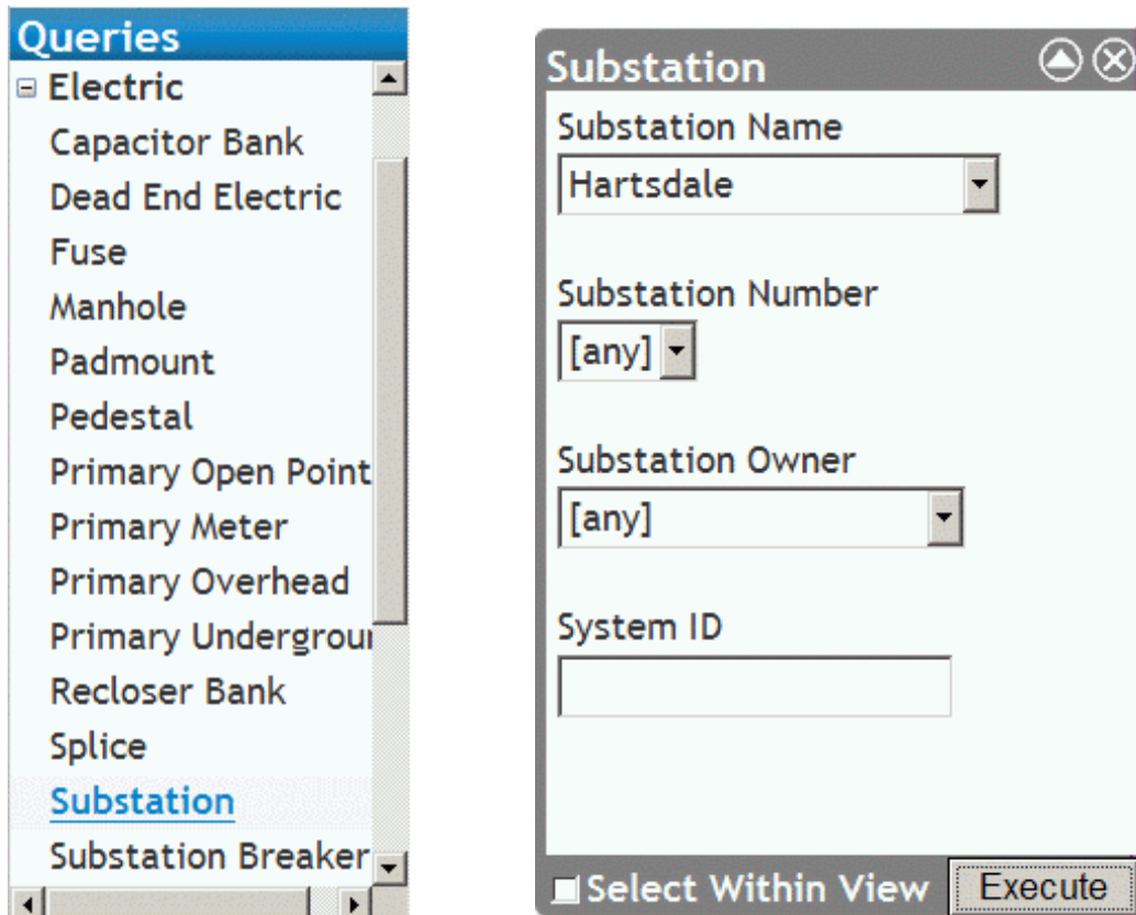
Figure 3.1-3. Query execution.
