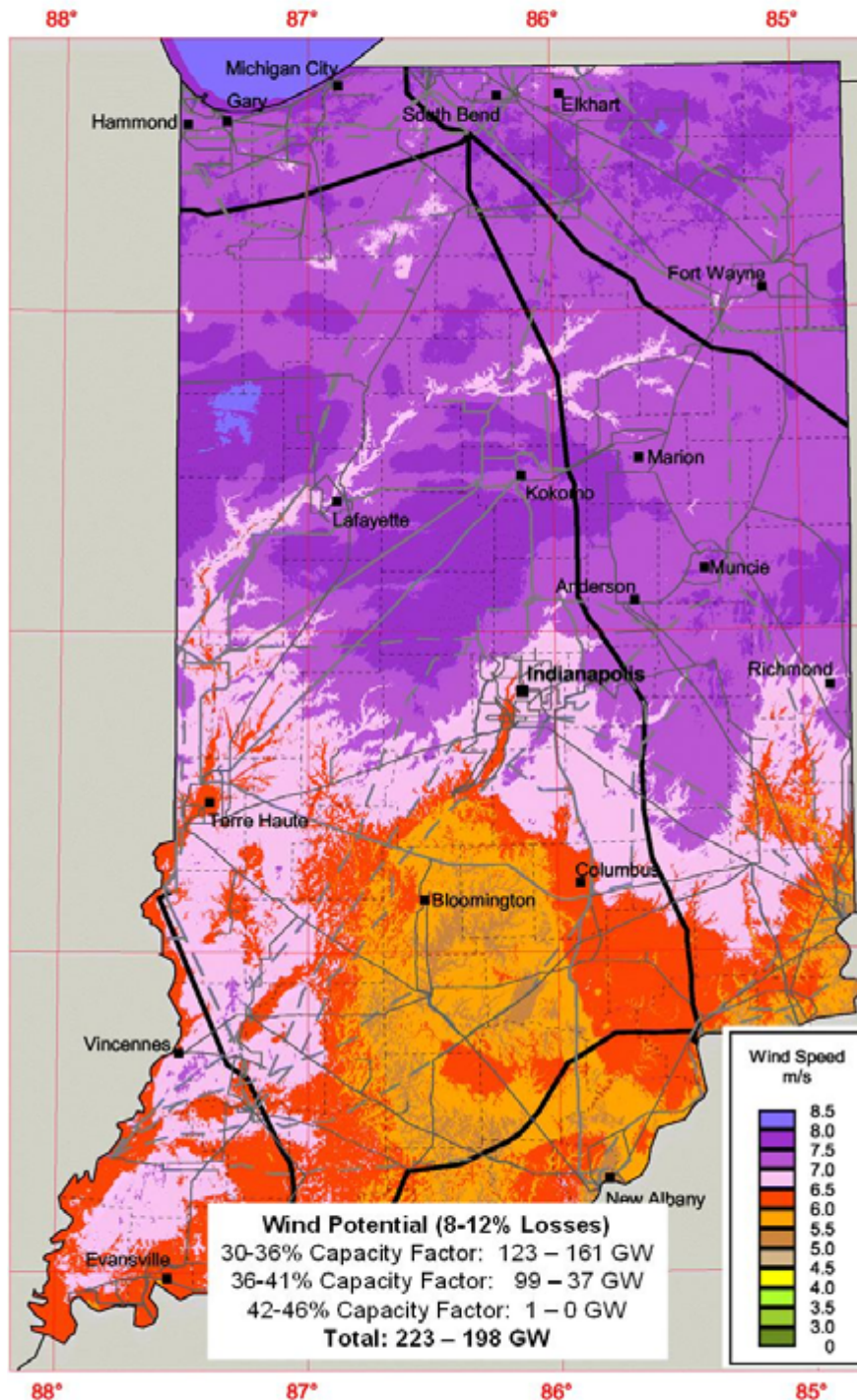
Figure 1.1.c. Indiana 70 meter wind speed map
