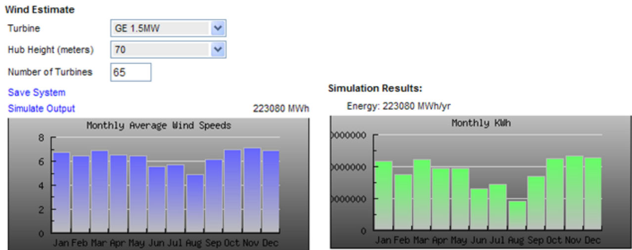
Figure 3.1.2.c. Area 1 – 65 tower, 100 MW, 70 m hub height simulation
