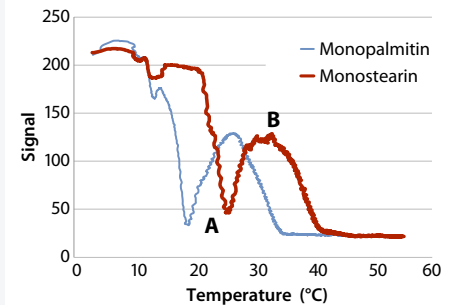
0.6% monostearin and 0.6% monopalmitin in tallow B100. The size and shape of the crystals change as the temperature is raised. These changes take place concurrently in the regions marked A and B.
