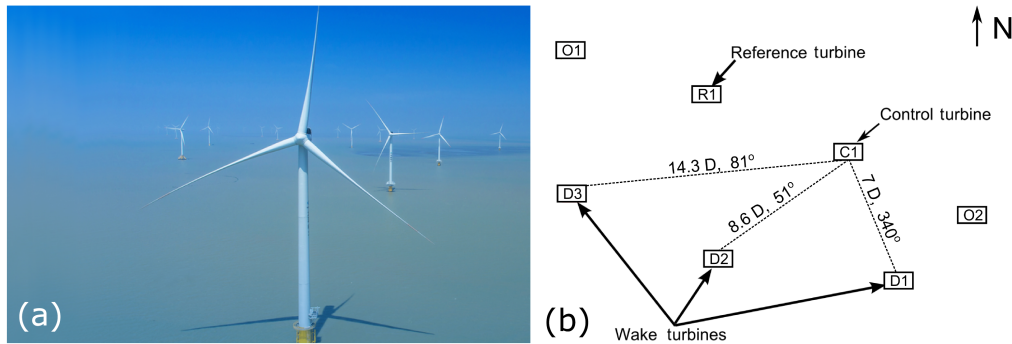
Figure 2. (a) Rudong wind farm used in the field study. (b) Turbine locations. The wake-steering control strategy is implemented to mitigate the wake interactions between C1, on the one hand, and D1, D2, and D3, on the other. As indicated by the diagram, C1 is the control turbine, R1 is the reference turbine, and D1, D2, and D3 are downstream turbines waked by C1. Turbines O1 and O2 are other turbines not directly used in the study but whose wakes are noticed in certain directions.
