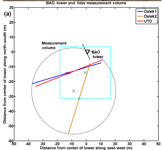
Figure 3. Top: schematic of the triple-Doppler virtual tower stares (VTS) of the three Leosphere 200S scanning lidars (Dalek1: blue, Dalek2: brown, and UTD: red), as they stare at the BAO tower's six levels of sonic anemometers at 50, 100, 150, 200, 250, and 300 m a.g.l. The WCv2 is also shown near the BAO tower. Bottom: bird's-eye view of the measurement volume (cyan box, with x at the center) resulting from the range gates of the three scanning lidars, drawn with circles at the centers of the beams, to scale. The footprint of the beams of the VTS is shown in the black circle, with an x at the center.
