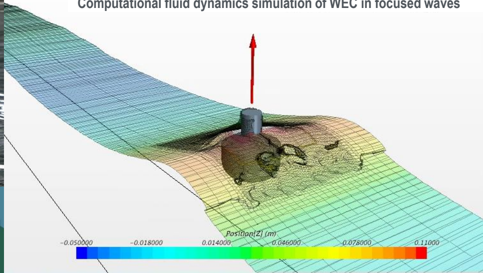
Computational fluid dynamics simulation of WEC in focused waves
