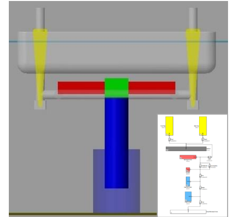
WEC-Sim numerical model of the experimental testing
