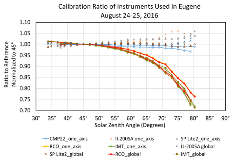
Fig. 2. Calibration comparison of instruments used in this study. The responsivities at 45° are used to normalize the calibrations.
