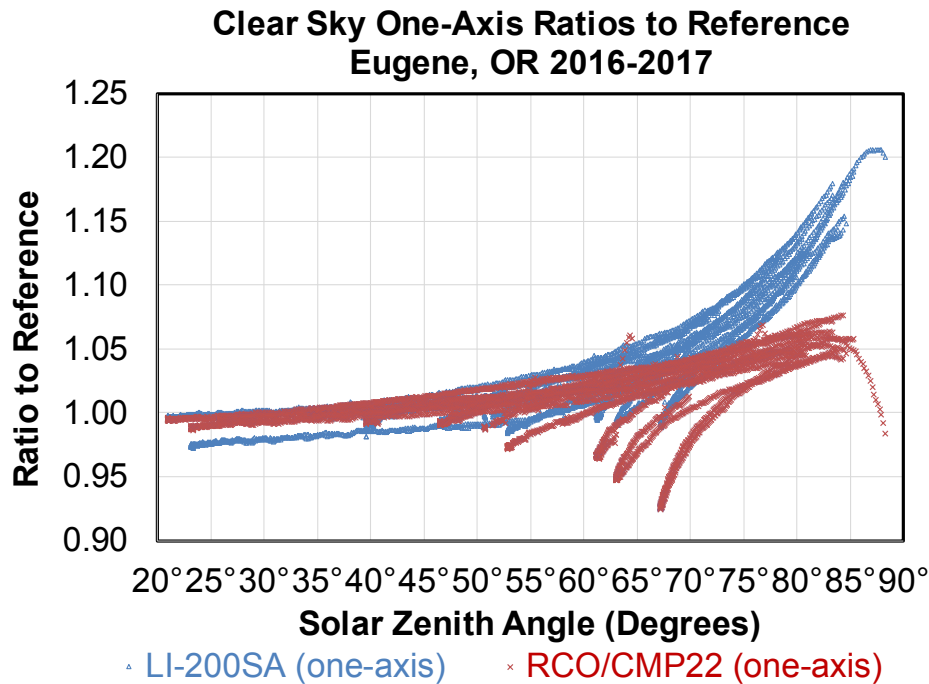
Fig. 6: Clear-sky ratio data between a LI-200S pyranometer and a RCO reference cell against the reference CMP 22 pyranometer. Clear-sky periods were shown for each month of the year.
