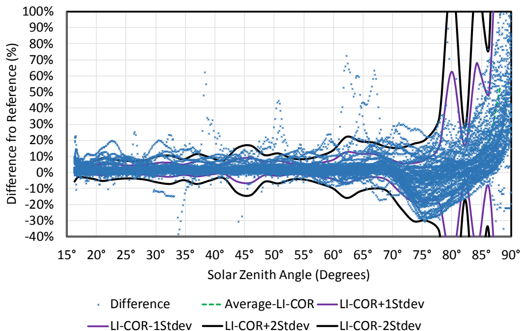
Fig. 8: Ratio of LI-200A measurements to those of the reference pyranometer in Golden, CO under all weather conditions in June, 2016. The dotted green line shows the average value and the thin purple lines show one standard deviation from the average. The thick black lines show the two standard deviations from the average. 95% of the data points should be within two standard deviations for a Gaussian distribution of the differences.
