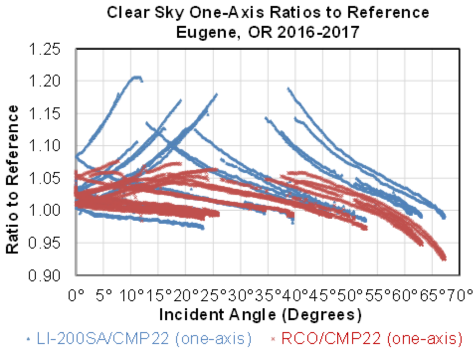
Fig. 7: Clear-sky ratio data between a LI-200A pyranometer and an RCO reference cell compared to the reference CMP 22 pyranometer plotted against the incident angle instead of SZA. Clear-sky periods are shown for each month of the year.
