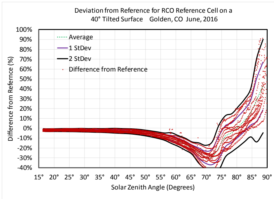
Fig. 5: Plot of the ratio of a RCO reference cell divided by the reference pyranometer measurements under clear-sky conditions in June, 2016 at Golden, CO.
