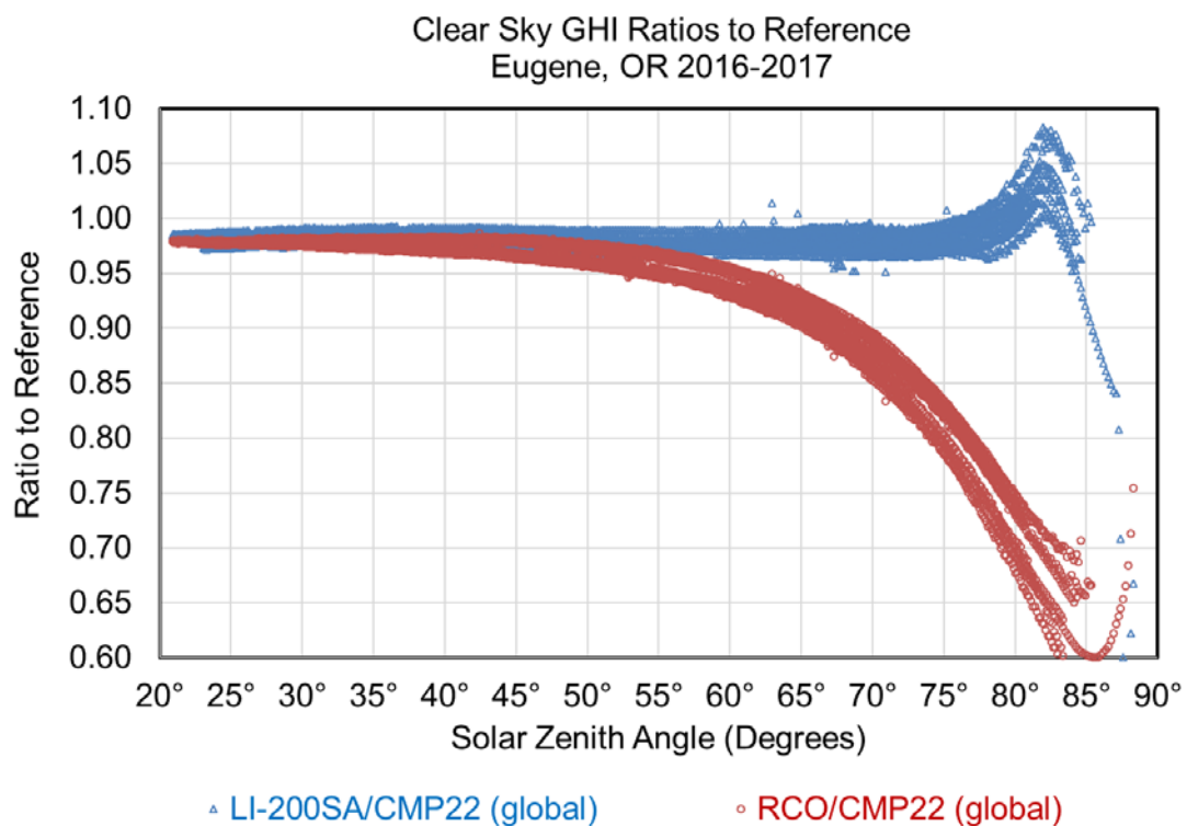
Fig. 3: Ratio of a LI-200SA pyranometer (blue triangles) and RCO reference cells (red circles) values divided by the values from the reference CMP 22 pyranometer on a horizontal surface during clear skies for selected days throughout the year at Eugene, Oregon.
