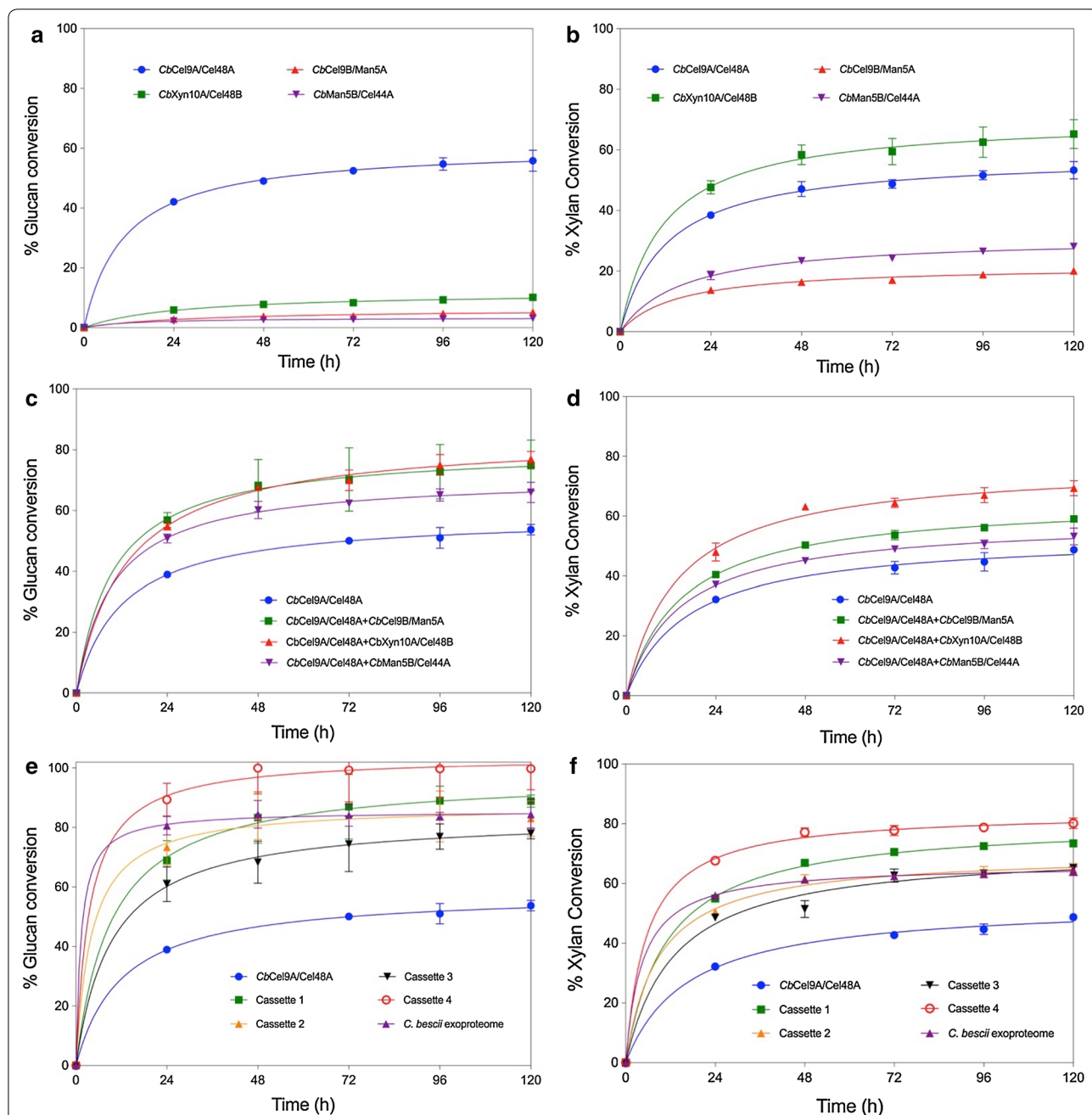
Fig. 5 APCS conversion by CbCel9A/Cel48A , CbCel9B/Man5A , CbXyn10A/Cel48B , and CbMan5B/Cel44A . a Glucan conversion of APCS by individual C. bescii enzymes, b xylan conversion of APCS by individual C. bescii enzymes, c glucan conversion of APCS by binary combinations of C. bescii enzymes, d xylan conversion of APCS by binary combinations of C. bescii enzymes, e glucan conversion of APCS by ternary and quaternary combinations of C. bescii enzymes, f Xylan conversion of APCS by ternary and quaternary combinations of C. bescii enzymes. Cassette 1 is a combination of CbCel9A/Cel48A , CbCel9B/Man5A , CbXyn10A/Cel48B , cassette 2 is a combination of CbCel9A/Cel48A , CbCel9B/Man5A , CbMan5B/Cel44A , cassette 3 is a combination of CbCel9A/Cel48A , CbXyn10A/Cel48B , CbMan5B/Cel44A , cassette 4 is a combination of CbCel9A/Cel48A , CbCel9B/Man5A , CbXyn10A/Cel48B , CbMan5B/Cel44A . All enzyme loadings can be found in the methods section and supplementary information (Additional file 1: Tables S4, S5)
