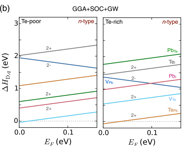
Fig. 5 Defect formation energy as a function of Fermi energy for vacancies, interstitials, and anti-site defects in PbTe, calculated with a HSE with SOC and band edge shifts from single step G_0W_0 , b GGA with SOC and band edge shifts from GW calculations. Pb and Te interstitial correspond to the tetrahedral interstitial site. HSE + SOC + G_0W_0 results correctly predict the intrinsic bi-polar conductivity in PbTe
