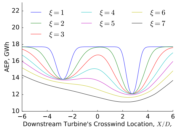
Figure 3 The impact of the wake relaxation factor, \xi . One turbine was moved across the wakes of two upstream turbines (see Fig. 2). [6]
