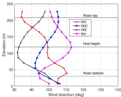
(a) Max veer profiles at R = 10 km
