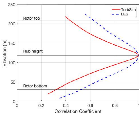
(a) Vertical correlation at R = 10 km
