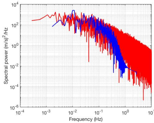
(c) Power spectral density at R = 15 km
