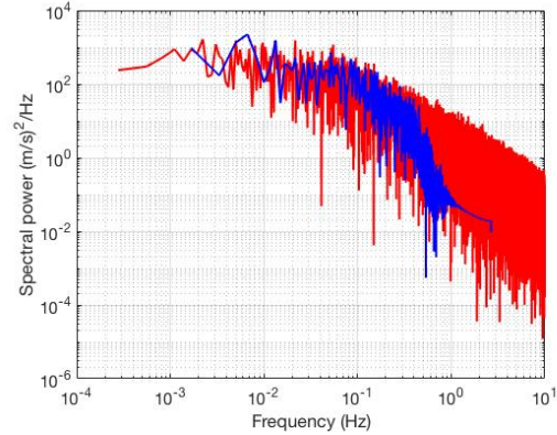
(b) Power spectral density at R = 12 km
