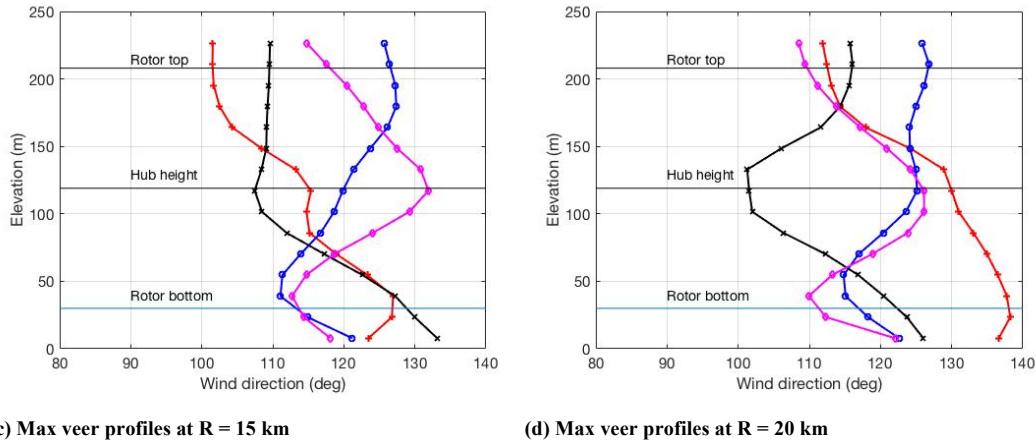
Figure 4: Maximum instantaneous veer profile for the four profile shapes at four radii from the hurricane center: (a) internal eyewall boundary R = 10 km, (b) inside eyewall R = 12 km, (c) external eyewall boundary R = 15 km and (d) outside of the eyewall R = 20 km. The hub height and rotor top and bottom of the theoretical DTU reference turbine, at elevations of 119m, 208 m and 30 m, respectively are indicated with horizontal lines.
