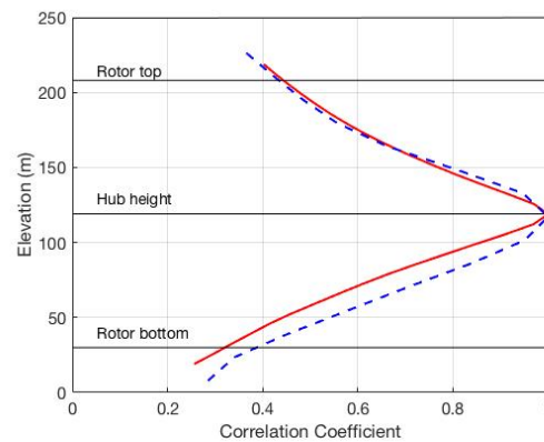
(b) Vertical correlation at R = 12 km
