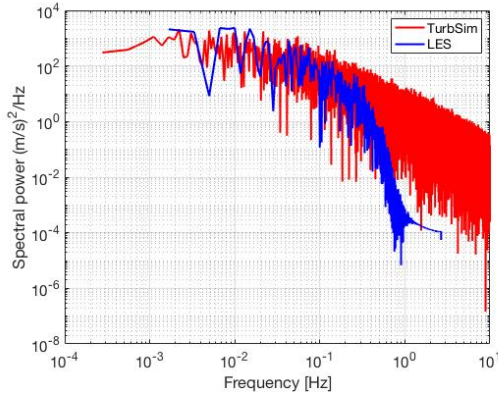
(a) Power spectral density at R = 10 km
