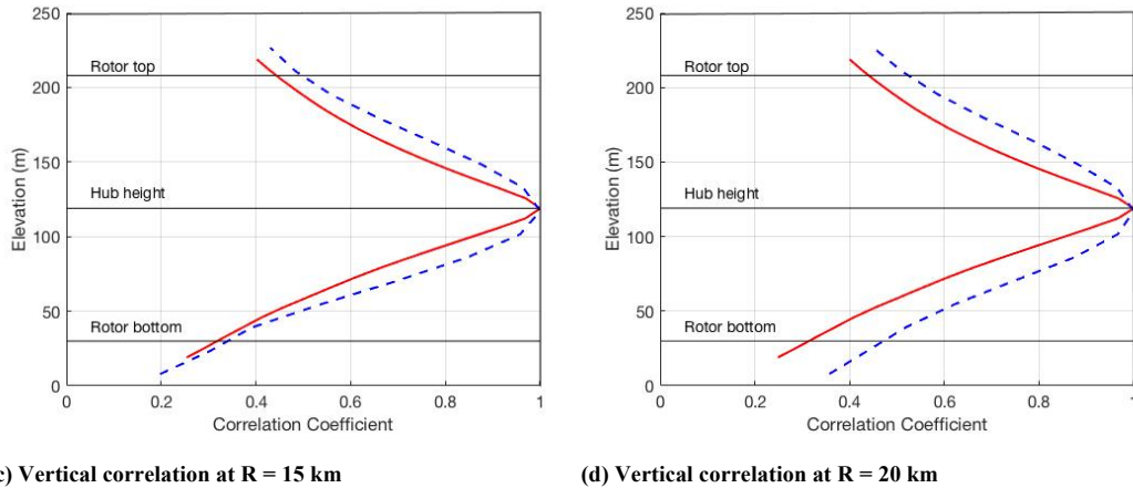
Figure 7: Profiles of correlation coefficient between the 10-min horizontal wind speed time series at each elevation and the 10-min horizontal wind speed time series at hub height for TurbSim (red) and LES (blue dashed) simulations, at four different radii from the hurricane center.
