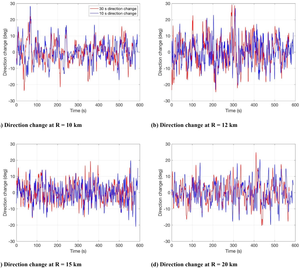
180 Figure 3: Time series of maximum wind direction change at various radii (R) of the hurricane at hub height: (a) inner 185 edge of eyewall R = 10 km, (b) inside eyewall R = 12 km, (c) outer edge of eyewall R = 15 km and (d) outside of the eyewall R = 20 km. The red and the blue lines represents the maximum wind direction change over moving intervals of 30 s (red) and 10 s (blue).
