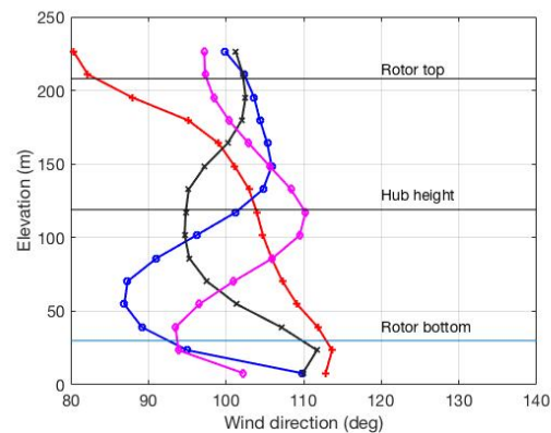
(b) Max veer profiles at R = 12 km
