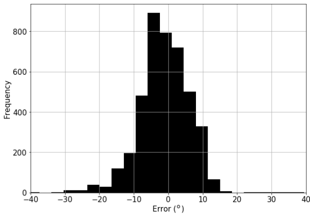
Figure 10. Error distribution of the estimated wind direction compared with measurements from the sodar. Note the measurements of the sodar are interpolated to match the 1 min time series from the consensus algorithm.
