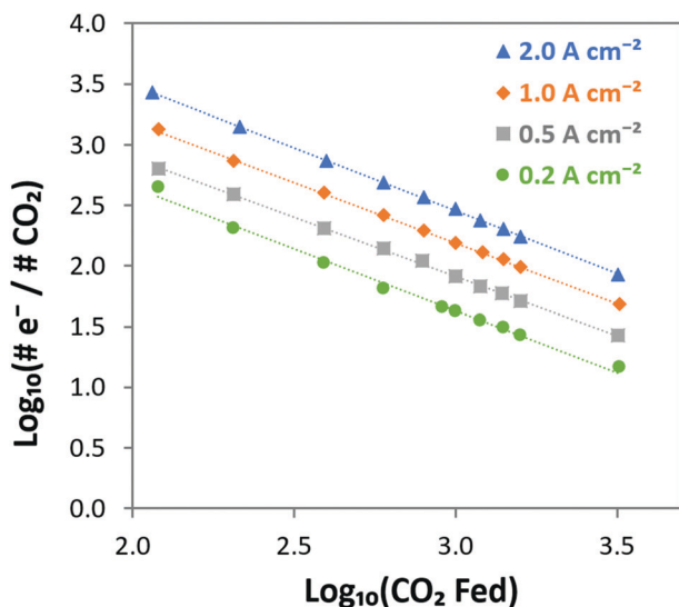
Fig. 4 Visualizing the steady-state transport of \text{CO}_2/\text{CO}_3^{2-} from the cathode to the anode in AEMFCs operating at 0.2, 0.5, 1 and 2 \text{ A cm}^{-2} at 60^\circ \text{C} over a wide range of \text{CO}_2 concentrations. The linear relationship with a slope of -1 verifies the relationship predicted in eqn (14) between the cathode \text{CO}_2 feed concentration and the portion of the charge that is carried by \text{CO}_3^{2-} , showing that \text{CO}_2 uptake and \text{CO}_3^{2-} incorporation is a Nernstian process and driven by the ORR.
