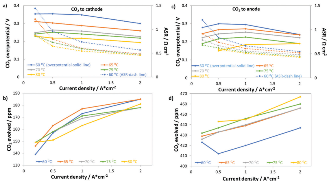
Fig. 7 Impact of temperature on the total \text{CO}_2 -related overpotential, ASR and anode \text{CO}_2 exhaust with 400 ppm \text{CO}_2 fed to the cathode at multiple current densities. Total \text{CO}_2 overpotential (solid lines) and ASR (dashed lines) when \text{CO}_2 was fed to the (a) cathode and (c) anode. \text{CO}_2 concentration in the anode effluent when \text{CO}_2 was fed to the (b) cathode and (d) anode. An LDPE–BTMA AEM (IEC = 2.5 mmol \text{g}^{-1} ) was used in these experiments.
