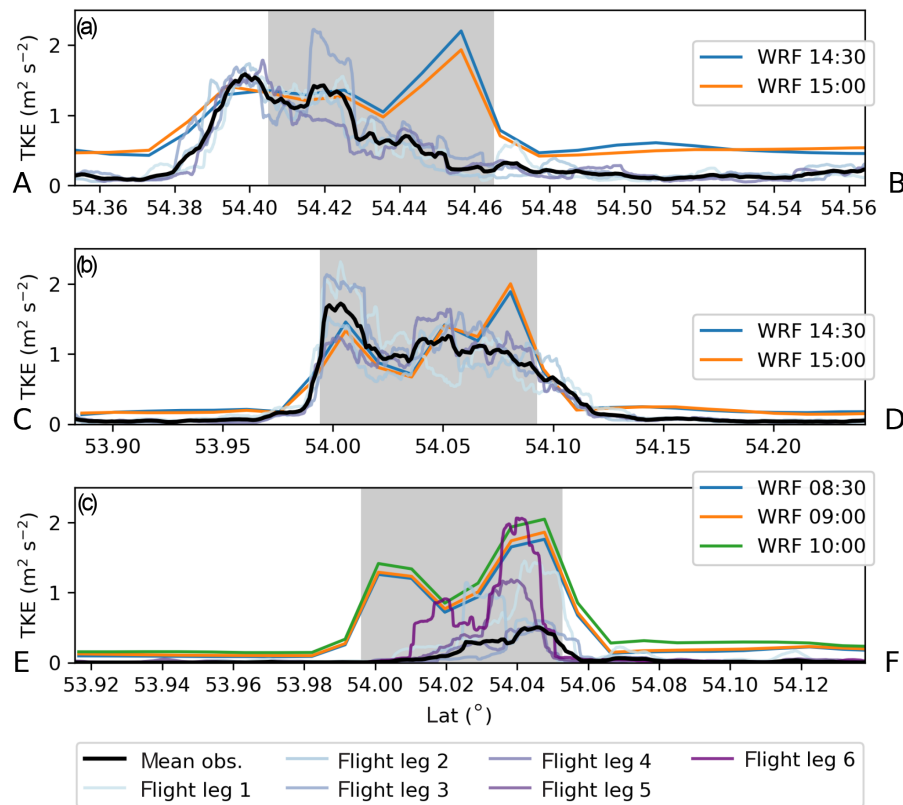
Figure 10. As in Fig. 8 but for the TKE.
