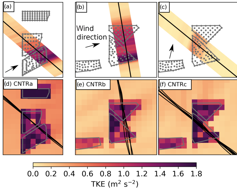
Figure 9. As in Fig. 7 but for the TKE.
