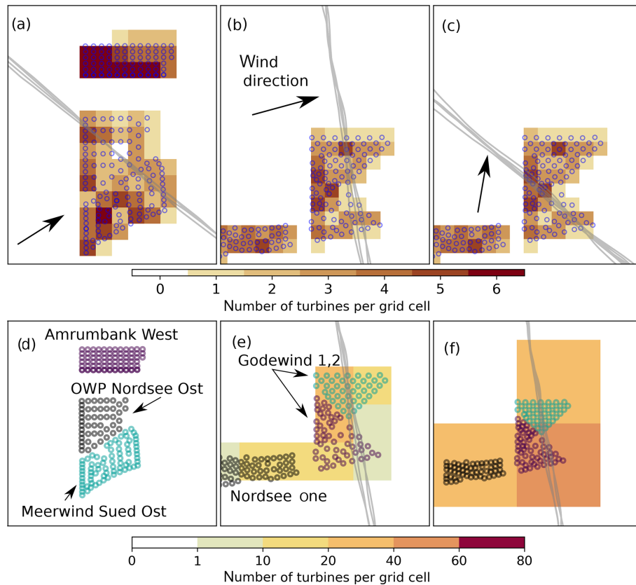
Figure 2. The number of wind turbines within one grid cell in colored contours for the wind farms: (a) Meerwind Süd Ost (MSO) and OWP Nordsee Ost (ONO) and (b–c) Godewind Wind 1, 2 (GW) for the control simulations (CNTRa, CNTRb, CNTRc). The size of the contour areas corresponds to the size of the horizontal model grid. The circles denote the exact locations of the single wind turbines, whereby the wind turbines are colored according to the wind farm they belong to in panels (d)–(f); additionally, panels (e)–(f) show the horizontal grid with 5 and 16 km resolution for the following sensitivity studies: DX5, DX16, DX5noTKESource and DX16noTKESource (see Table 2 for an overview of all simulations). The wind turbines are not colored in panels (a)–(c) for better visibility of the wind turbine density. The gray lines denote the flight track of the research aircraft.
