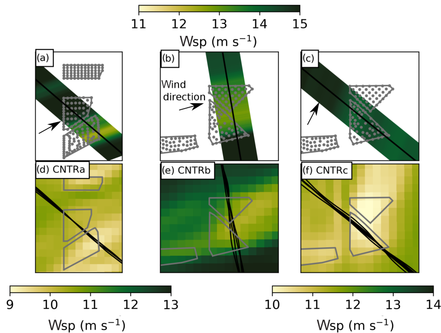
Figure 7. Plan view on observed (a–c) and simulated (d–f) horizontal wind speed at 14:30, 15:00 and 09:00 UTC on 9 August, 14 and 15 October 2017, respectively, with horizontal wind speed in colored contours at 200 (a, d) and 250 m a.s.l. (b, c, e, f). Black lines denote the flight path over the wind farms. The observations show the mean of the observed wind speed, similar to Fig. 8a–c. The locations of wind farms and single wind turbines are shown in gray polygons and dots, respectively. Each column corresponds to one case study (e.g., panels a and d correspond to the measurements taken on 9 August 2017). The wind direction is denoted by the black arrow as retrieved by the aircraft observations.
