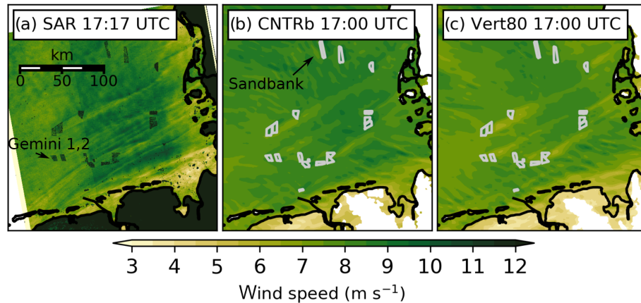
Figure 4. A comparison of SAR from Copernicus Sentinel-1A and WRF retrieved wind speed at 17:17 and 17:00 UTC, respectively, on 14 October 2017 (case study II). The SAR data show the wind speed at 10 m, whereas the model output is taken from the model level closest to 10 m. Therefore, we show the wind speed at 17 and 15 m for the CNTR and Vert80 simulations, respectively. The grayish polygons (b–c) denote the locations of the wind farms.
