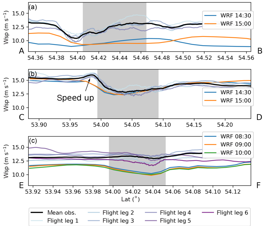
Figure 8. Observed (thin blue and purplish lines; the purple amount is increased based on how late the flight leg was flown) and simulated wind speed interpolated onto the flight track, as shown in Figs. 1 and 2 for the three case studies (a–c) as indicated in Table 1. Note the mean speed is more or less perpendicular to the flight legs (see Fig. 7a, b, c); hence, the mean wind speed points into the paper plane. The thick black line shows the mean of all wind speed measurements over the wind farms similar to the measurements shown in Fig. 7a–c. The gray shaded areas denote the location of the wind farm. The capital letters on the x axis show the orientation of the axis as indicated in Fig. 1.
