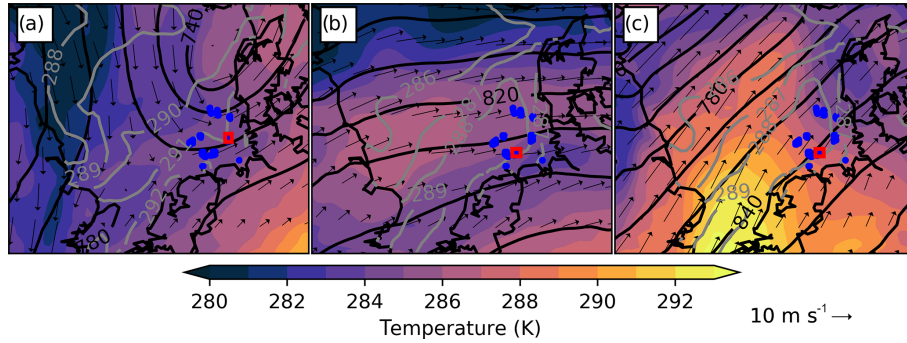
Figure 5. ERA5 reanalysis data: temperature (colored contours; K) and geopotential height (20 m increments) as black contour lines at 925 hPa for the three case studies as listed in Table 1, at 15:00 UTC on 9 August 2017, at 15:00 UTC on 14 October 2017 and at 09:00 UTC on 15 October 2017 (Table 1). The gray solid contour lines show the SST.
