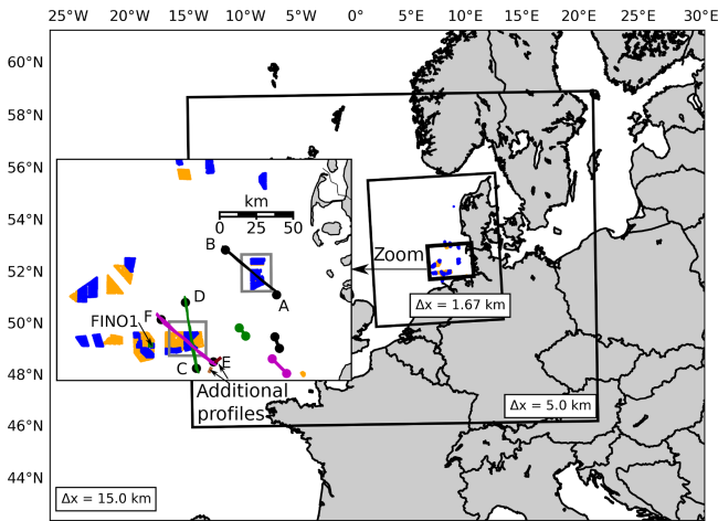
Figure 1. Locations of WRF domains and wind farms at the North Sea. A close-up on the German Bight shows the wind farms of interest framed with gray rectangles and the flight tracks of the three measurements in black, green and magenta, corresponding to the measurements executed on 9 August, 14 and 15 October 2017, respectively. All measurements over the wind farms have a start and end point indicated with a capital letter for better orientation in Figs. 8, 10 and 11. Blue wind farms are operational; orange wind farms are approved or under construction during the time period investigated in this study. The thick lines indicate the locations of the climb flights, whereby the coloring corresponds to the coloring of the flight tracks over the wind farms, except the light red and red thick line showing the two additional profiles (see annotations) before and after the two additional flight legs. A detailed look (close-up on gray rectangles) at the wind turbine distribution of the wind farms of interest is provided in Fig. 2. The wind turbine location data were provided by the German Federal Maritime and Hydrographic Agency (BSH) and Bundesnetzagentur (2019).
