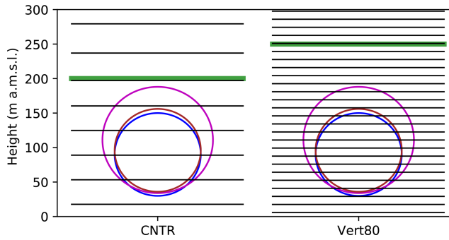
Figure 3. Distribution of the vertical levels with height and the levels intersecting with the rotor areas of the two wind turbine types used in the wind farms, as listed in Table 3 for the CNTR and Vert80 simulations. The rotor areas of the wind turbines SIEMENS-SWT-6.0-154, SIEMENS SWT 3.6-120 and SENVION 6.2 are shown in magenta, blue and red, respectively. The green lines denote flight heights at 200 and 250 m a.m.s.l., which is necessary due to the different wind turbine heights.
