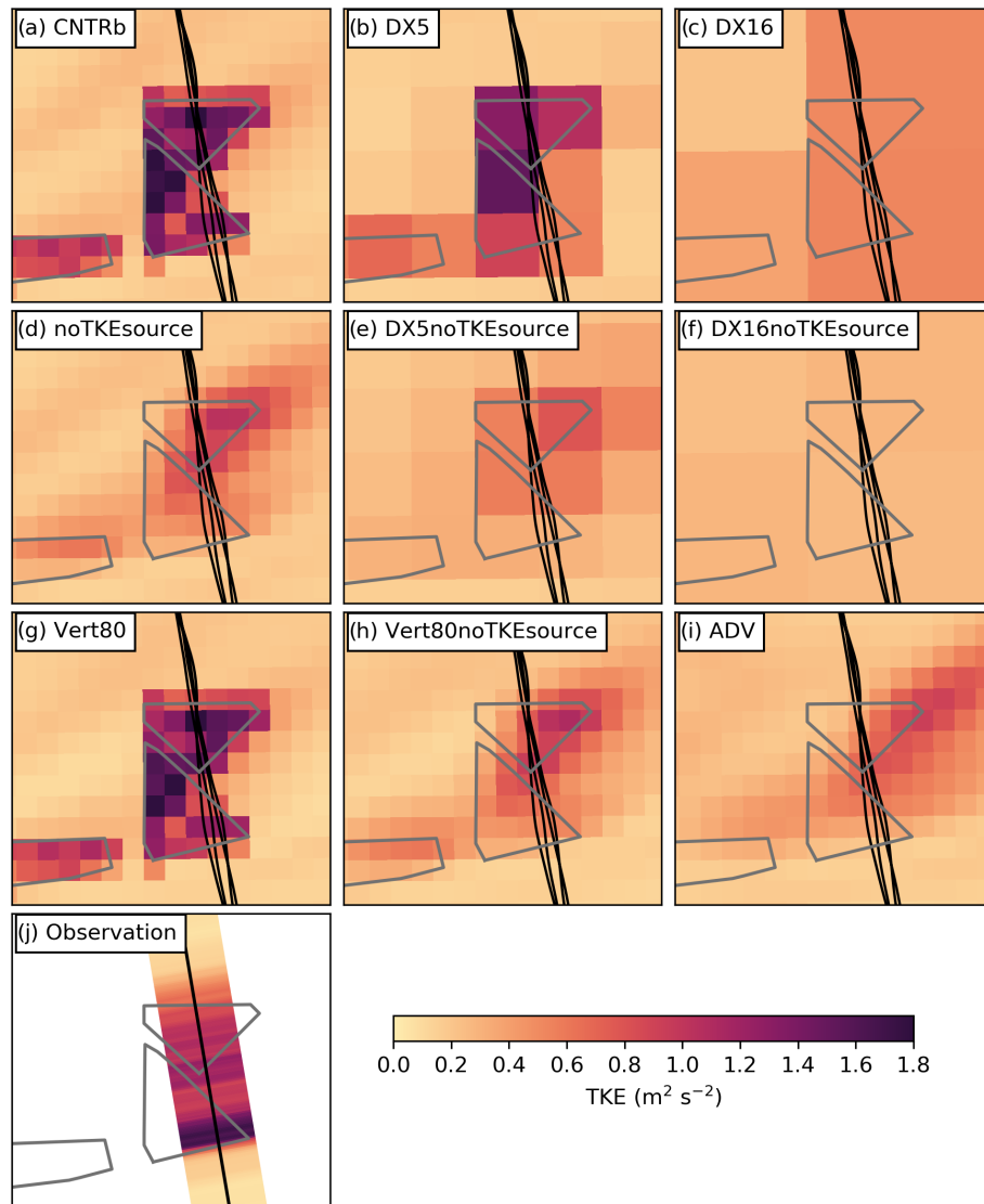
Figure 12. As in Fig. 9 but for the sensitivity simulations (b–i) DX5, DX16, noTKESource, DX5noTKESource, DX16noTKESource, Vert80, Vert80noTKESource and ADV at 15:00 UTC. A summary of all sensitivity tests is listed in Table 2. For better comparison, the control simulation CNTRb is shown in panel (a) and the observations in (j).
