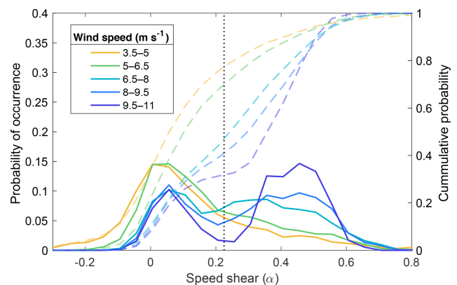
Figure 12. Speed shear probability density (solid lines) and cumulative (dashed lines) distributions for 1.5 \text{ m s}^{-1} wind speed regimes. The black dotted line marks \alpha = 0.225 .
