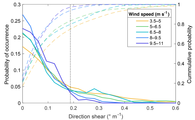
Figure 11. Directional wind shear probability density (solid lines) and cumulative (dashed lines) distributions for 1.5 \text{ m s}^{-1} wind speed regimes. The black dotted line marks 0.1875^{\circ} \text{ m}^{-1} of directional wind shear.
