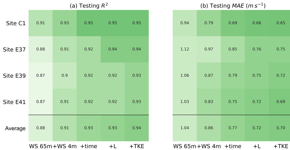
Figure 6. Testing R^2 and MAE in predicting the 30 min average wind speed at 143 m a.g.l. for the different sites and input feature combinations.
