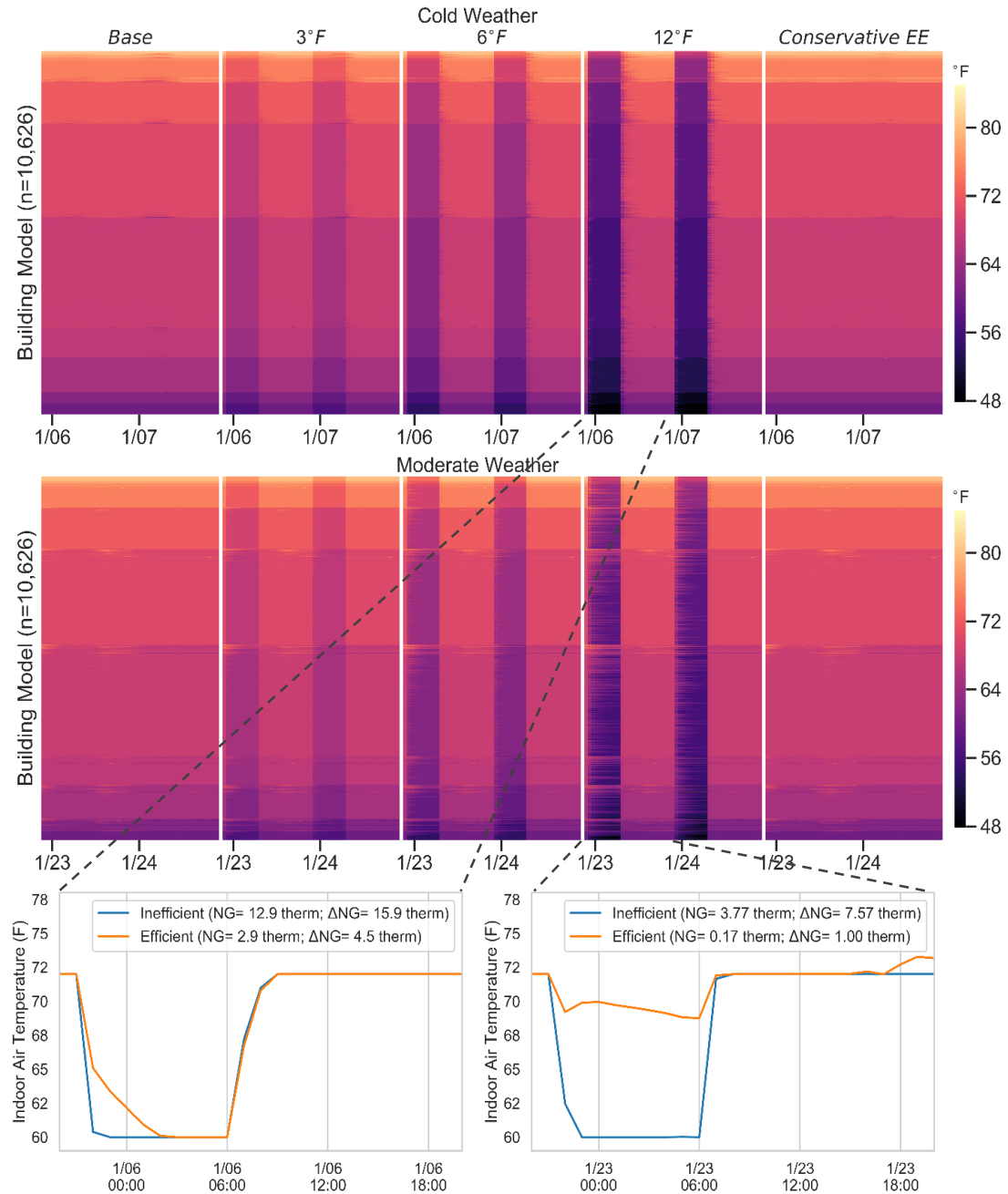
Figure 9. Heatmap of indoor air temperatures for the conservative approach during cold temperature (top) and moderate temperature (bottom) periods in 2018. The y-axis contains each building model for which the conservative setback was applied (46% of homes) and is sorted by average indoor air temperature. The lower two plots show expanded views of indoor air temperatures for two homes over 24 h during the cold period (left) and the mild period (right). One model is well insulated and tightly sealed (“Efficient”) and the other is poorly insulated and poorly sealed (“Inefficient”).
