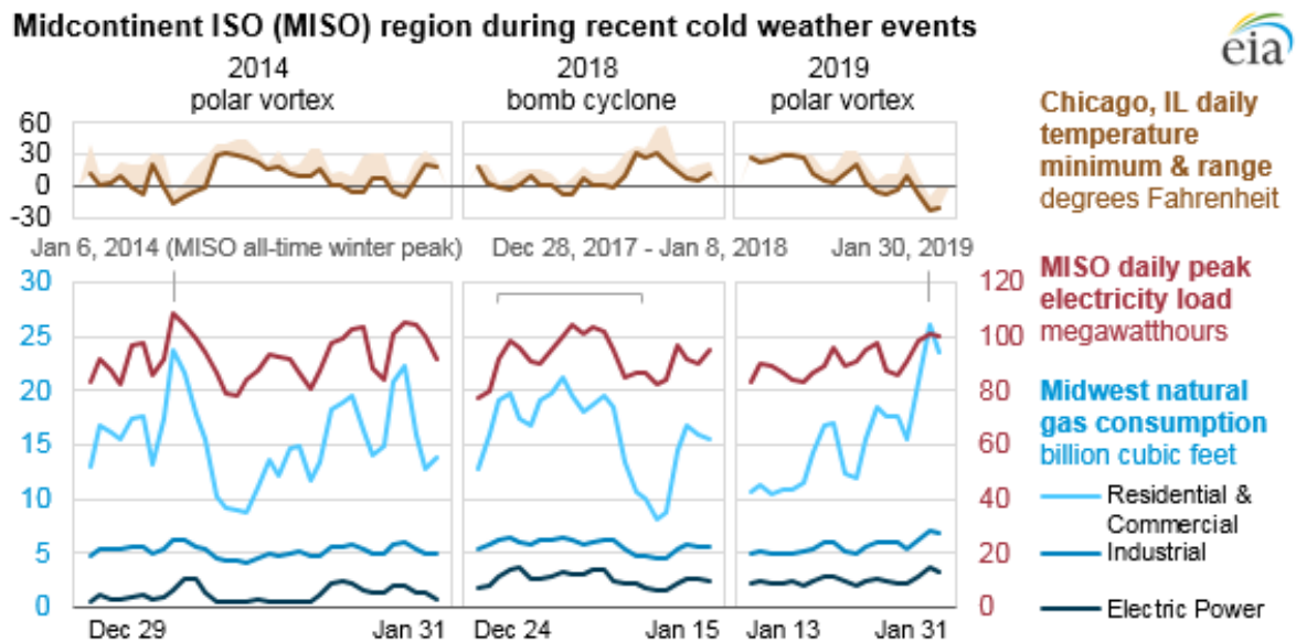
Figure 1. Historical temperature, electricity load, and natural gas consumption data for periods of extreme winter weather in the Midwest United States. Periods of extreme cold correspond with an increase in electricity and natural gas demand, which is primarily driven by residential and commercial heating. Source: U.S. Energy Information Administration [6].
