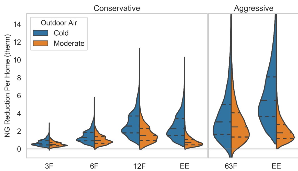
Figure 8. Distributions of total natural gas (NG) reductions from demand response and energy efficient upgrade scenarios from the cold and moderate weather baseline scenarios. Quartiles are represented by the lines inside each plot. The conservative plot displays all modeled homes, while the aggressive plot displays approximately 98% of the modeled homes, omitting extreme high and low data points.
