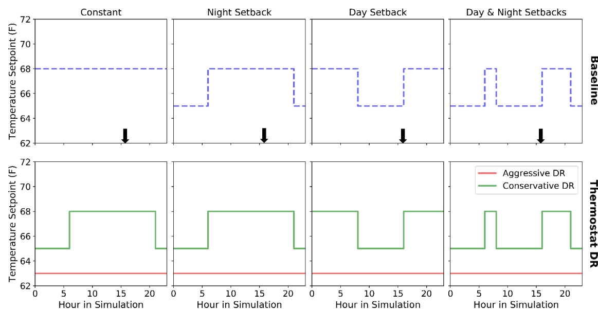
Figure 4. Example thermostat schedules for the baseline operation (top) and the resulting schedule after thermostat demand response (bottom).
