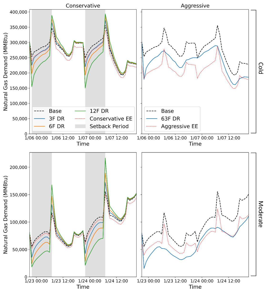
Figure 7. Total natural gas demand for heating during cold ( top ) and moderate ( bottom ) periods in 2018. Demand response (DR) and energy efficiency (EE) measures are applied to 46% of homes in the conservative scenario, and 94% of homes in the aggressive scenario. The sharp peaks and valleys shown in baseline, conservative, and energy efficiency profiles are a result of heating setbacks across homes that occur at the same time each day (i.e., not staggered).
