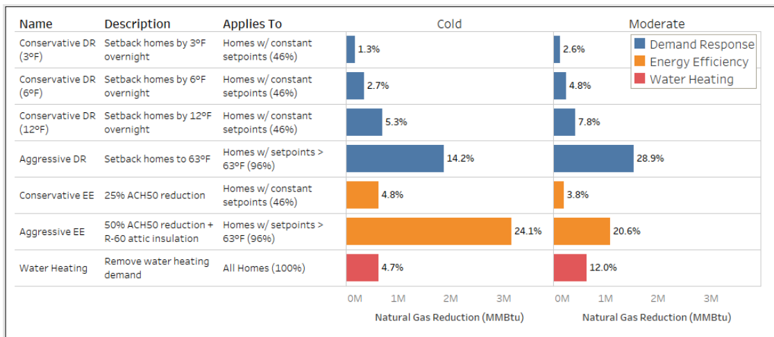
Figure 6. Total natural gas reduction from the baselines across 48 h periods of cold and moderate outdoor temperatures. The percentage of homes in which each case applies is shown in parenthesis in the “Applies To” column. The percentages shown at the end of each bar are the reductions in total natural gas demand from the baseline. The cold period refers to 5 January 2018–7 January 2018, coinciding with the bomb cyclone, and the moderate period refers to 22 January 2018–24 January 2018. ACH50 is the air changes per hour at 50 pascals pressure differential, a measure of the level of air sealing in a home.
