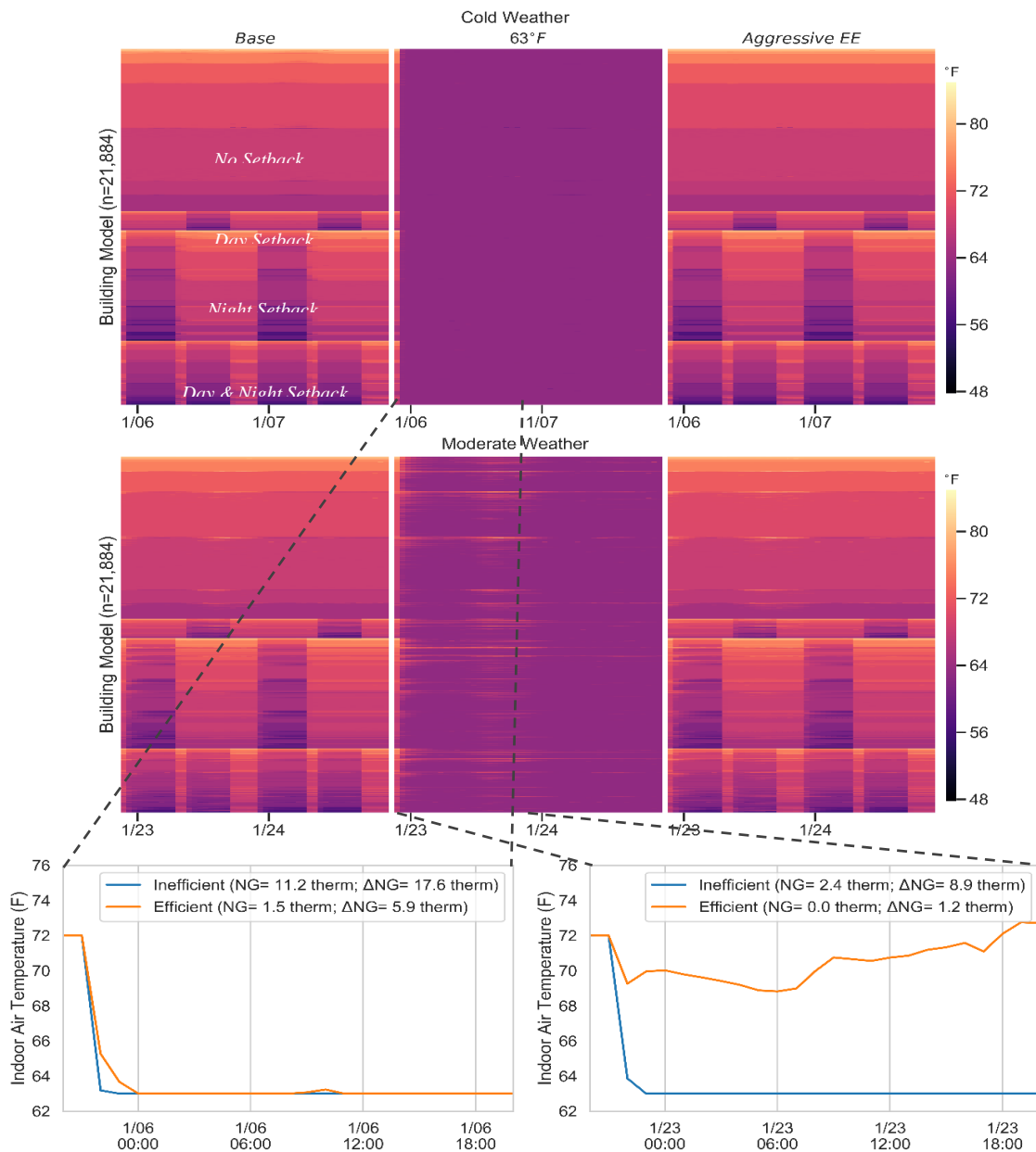
Figure 10. Heatmap of indoor air temperatures for the aggressive approach during cold temperature (top) and moderate temperature (bottom) periods in 2018. The y-axis contains each building model for which the aggressive setback was applied (94% of homes), and is sorted by existing setback and average indoor air temperature. The lower two plots show expanded views of indoor air temperatures for two homes over 24 h during the cold period (left) and the mild period (right). One model is well insulated and tightly sealed (“Efficient”) and the other is poorly insulated and poorly sealed (“Inefficient”).
