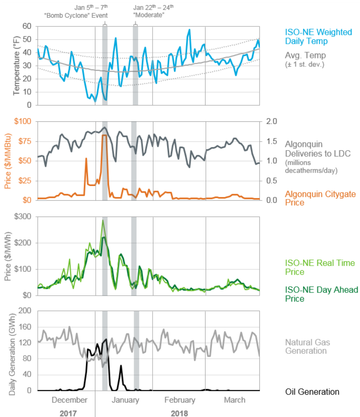
Figure 2. Summary statistics for the New England region for the winter of 2017–2018, highlighting temperatures (top panel), natural gas deliveries to local distribution companies (LDC) and prices on the Algonquin pipeline (second panel from top), daily average electricity prices in ISO-NE (third from top), and daily natural gas and oil generation (bottom). The bomb cyclone and moderate periods highlighted were selected for detailed modeling in this report. Data compiled from ISO-NE [37].
