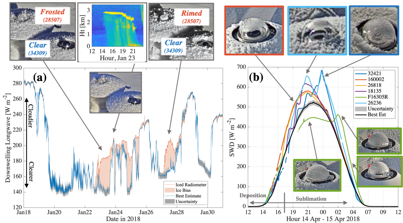
Figure 4. Case studies of icing for LWD in late January (a) and SWD during a clear day in April (b). Inset images show the condition of highlighted radiometers. The upper-center panel in (a) shows backscatter from the DoE-ARM ceilometer.
