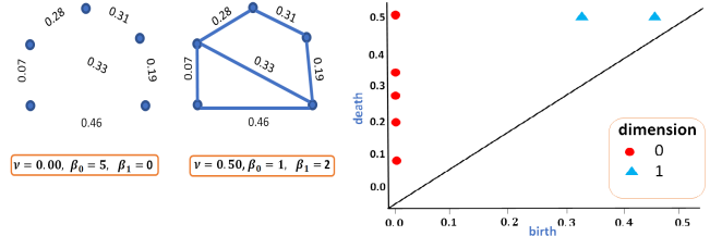
Figure 2: Illustration of Betti number ( \beta_0, \beta_1 ) estimation and persistence diagram for VR-filtration.
