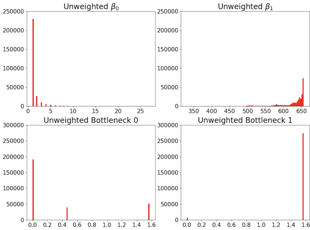
Figure 5: Histograms of Betti numbers and bottleneck distances in the contingency dataset.
