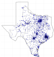
Figure 3: Map of the ACTIVSg2000 synthetic power system (Birchfield et al. 2017).
