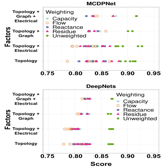
Figure 9: Score for amount of variance explained by two regression models (MCDPNet versus DeepNets) for different edge-weighting schemes and independent-variable subsets.
