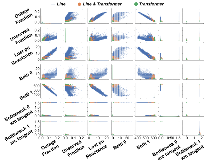
Figure 6: Scatterplot of the relationship between dependent variable (fraction of load not served, shown in the second row and second column) and independent variables in the contingency dataset under the electrical-distance weighting scheme.
