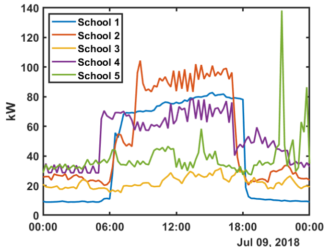
FIGURE 7. Measured 15-minute time series load profile for each building on July 9, 2018.
