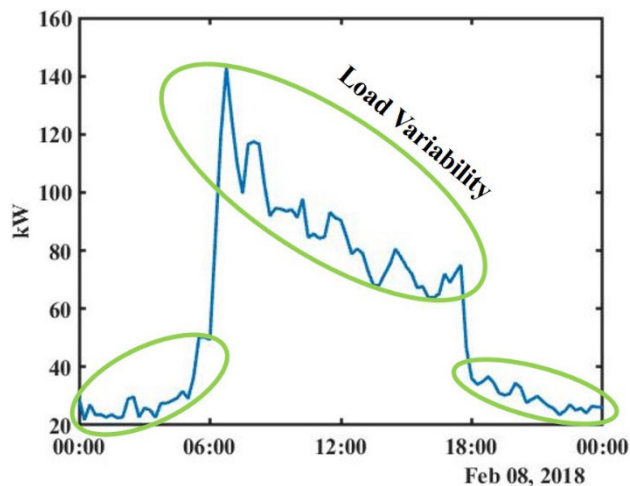
FIGURE 13. Measured commercial building load profile: February 8, 2018, sample day.
