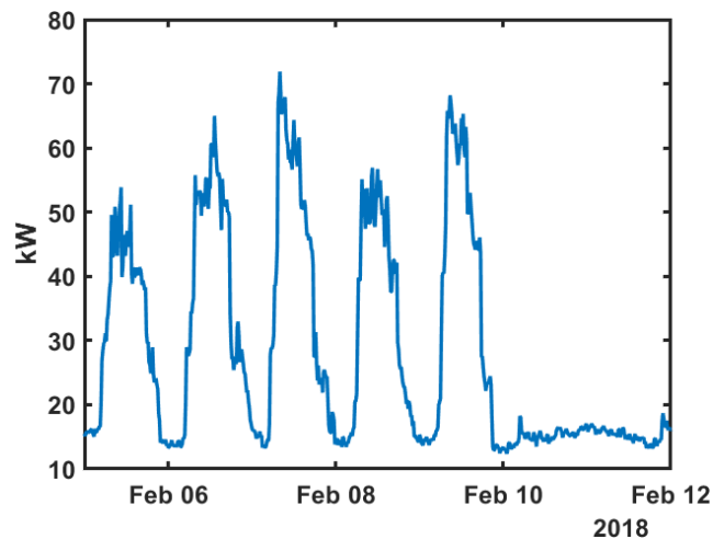
FIGURE 11. Measured commercial building load profile for one week, Feb 5–12, 2018.
