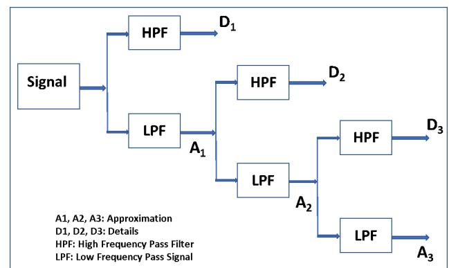
FIGURE 2. A three-level discrete wavelet transform.
