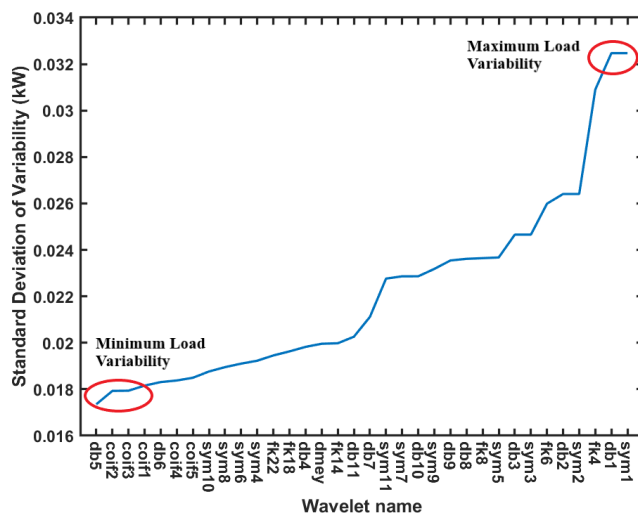
FIGURE 22. Increasing amounts of variability extracted with various wavelet functions at level 1, extracted from a measured commercial building load profile for one day: February 8, 2018.
