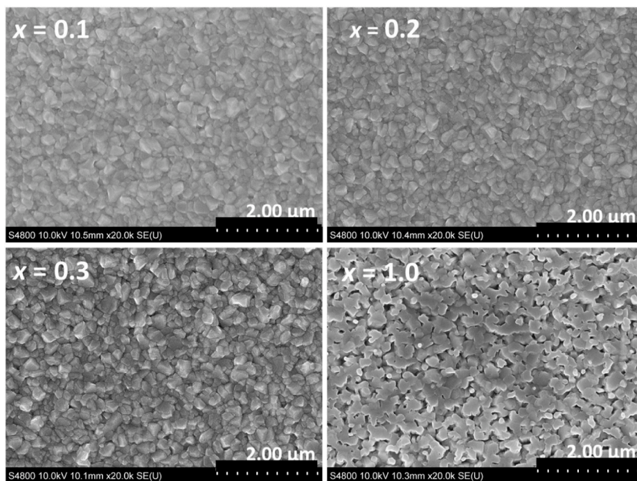
Fig. 2. Plan-view (SEM) of selected Cd(Se,Te) thin films (380 nm thick).
