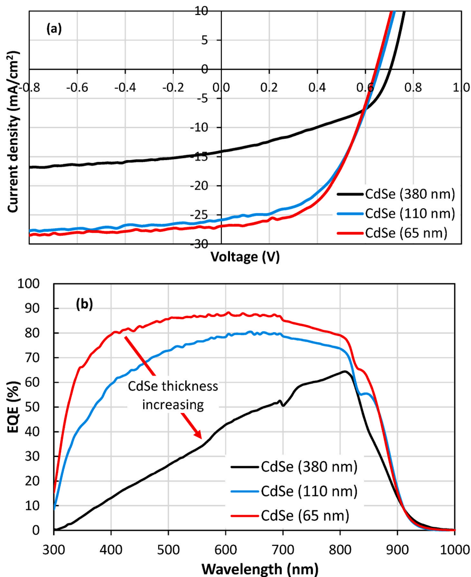
Fig. 5. Under illumination J-V curves (a) and EQE spectra (b) of FTO/SnO 2 /CdSe/CdTe:As devices.
