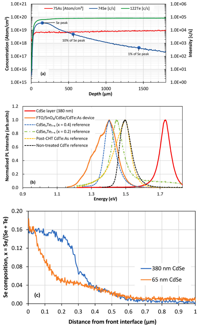
Fig. 7. Se, As, and Te SIMS profiles (a) and front-interface PL spectrum (b) of a FTO/SnO 2 /CdSe/CdTe:As device utilising 380 nm CdSe; PL spectrum of the 380 nm CdSe layer as well as reference films of as-deposited (undoped) CdTe, CHT arsenic doped CdTe, and an as-deposited (undoped) Cd(Se,Te) ( x = 0.4 , x = 0.2 ) alloy are also shown. (c) TEM/EDX Se line profile for devices utilising 65 and 380 nm CdSe.
