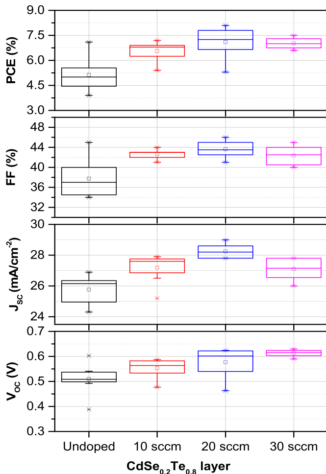
Fig. 10. Box plot comparison of J-V parameters of FTO/SnO 2 /CdSe/CdSe 0.2 Te 0.8 /CdTe:As devices (8 cells per device) with undoped and As doped Cd(Se, Te).
