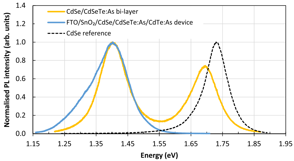
Fig. 8. Front interface PL spectrum of a FTO/SnO 2 /CdSe/CdSe 0.2 Te 0.8 :As/CdTe:As device in comparison to the PL spectrum of CdSe/CdSe 0.2 Te 0.8 :As bilayer and a reference CdSe film.
