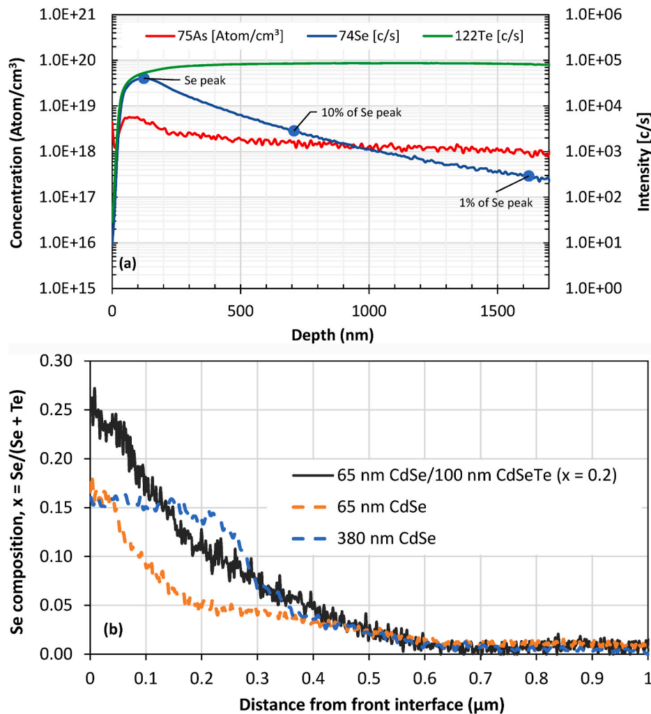
Fig. 13. (a) SIMS depth profiles for Se, As, and Te of the FTO/SnO 2 /CdSe/CdSe 0.2 Te 0.8 /CdTe:As device with 20 sccm As-doped Cd(Se, Te). (b) The STEM/EDX Se line profile for the FTO/SnO 2 /CdSe/CdSe 0.2 Te 0.8 /CdTe:As device with 10 sccm As-doped Cd(Se,Te), compared to devices utilising single CdSe layers of 65 and 380 nm.
