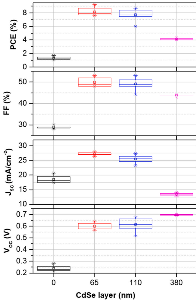
Fig. 6. Box plot comparison of J-V parameters of FTO/SnO 2 /CdSe/CdTe:As devices (8 cells per device) with varying thickness of CdSe.
