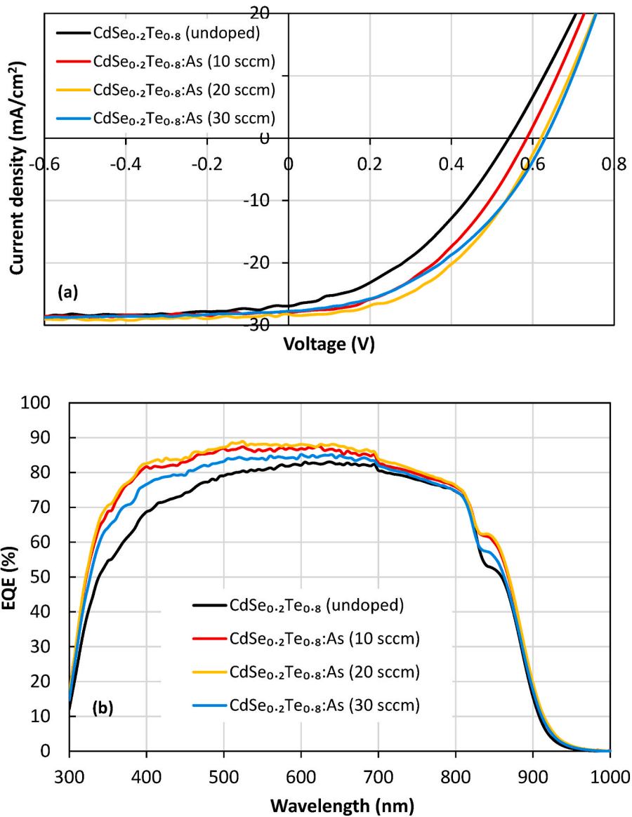
Fig. 9. Light J-V curves (a) and EQE spectra (b) of FTO/SnO 2 /CdSe/CdSe 0.2 Te 0.8 /CdTe:As devices with undoped and As doped Cd(Se,Te).
