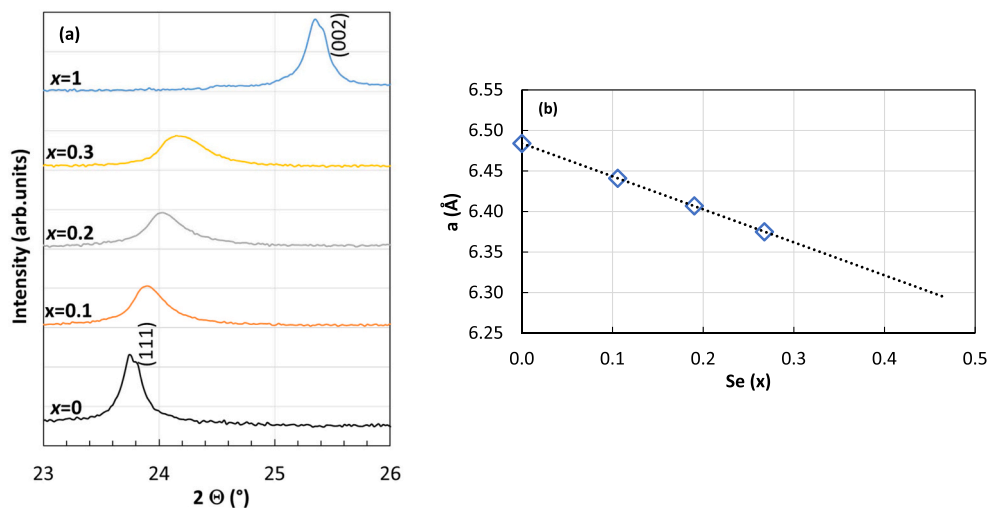
Fig. 3. (a) XRD spectrum of selected Cd(Se,Te) thin films (expanded view around the dominant (111) and (002) peaks for cubic and hexagonal phases, respectively). (b) Variation of the lattice constant with Se content for cubic films ( 0 \leq x \leq 0.3 ).
