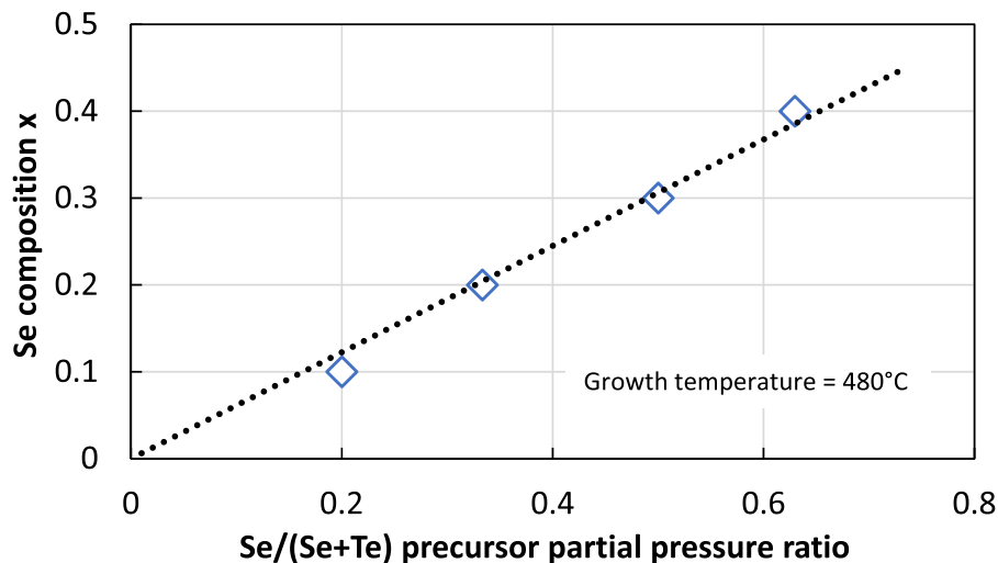
Fig. 1. Measured Se composition ( x ) as a function of the Se/(Se + Te) precursor partial pressure ratio.
