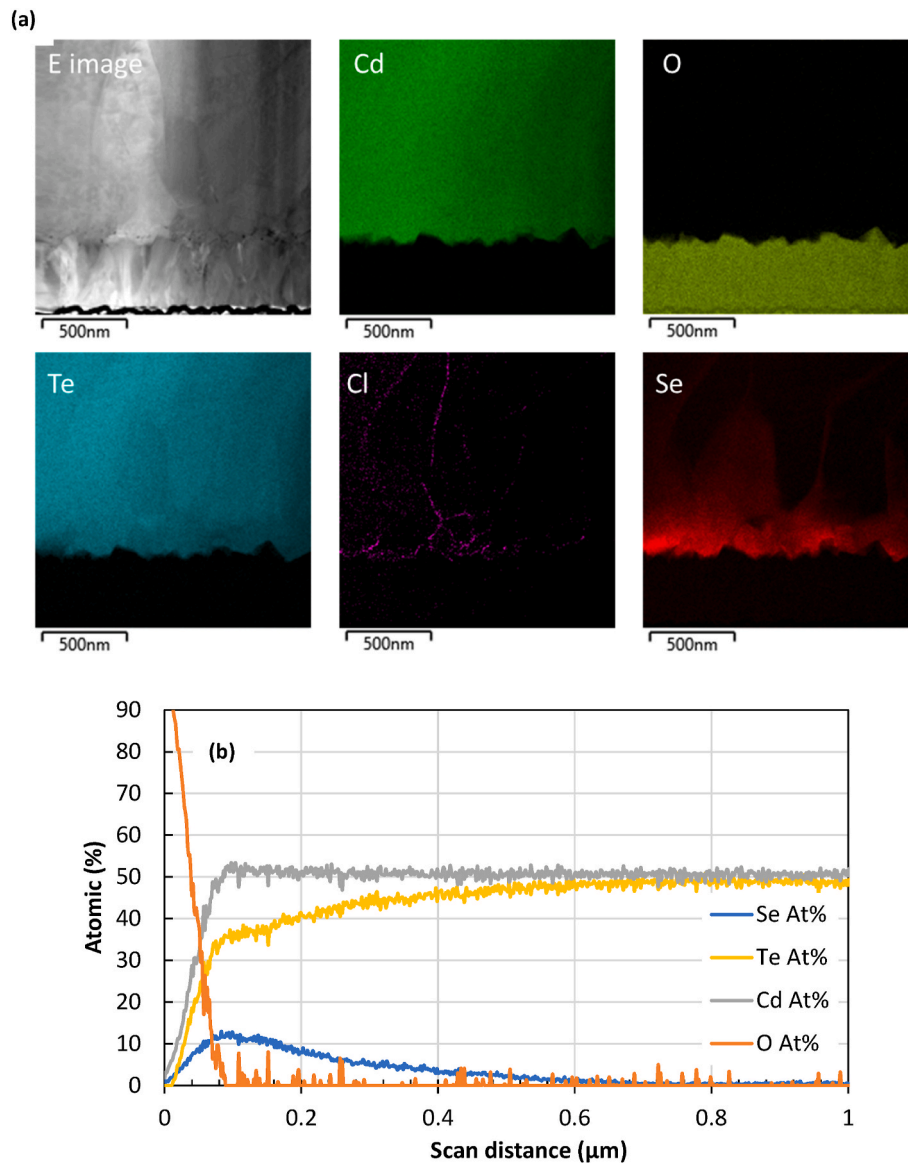
Fig. 12. Cross section STEM images with EDS maps for Cd, O, Te, Cl and Se (a) and cross sectional EDS line scans for Se, Te, Cd, and O (b) in a FTO/SnO 2 /CdSe/CdSe 0.2 Te 0.8 :As/CdTe:As device.
