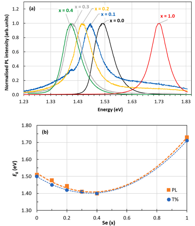
Fig. 4. (a) Micro-PL spectrum of Cd(Se,Te) thin films with x = 0 (CdTe), 0.1, 0.2, 0.3, 0.4 and 1 (CdSe), and (b) E_g (from Tauc plots and PL spectrum) vs. composition ( x ). The broken lines are polynomial fits.
