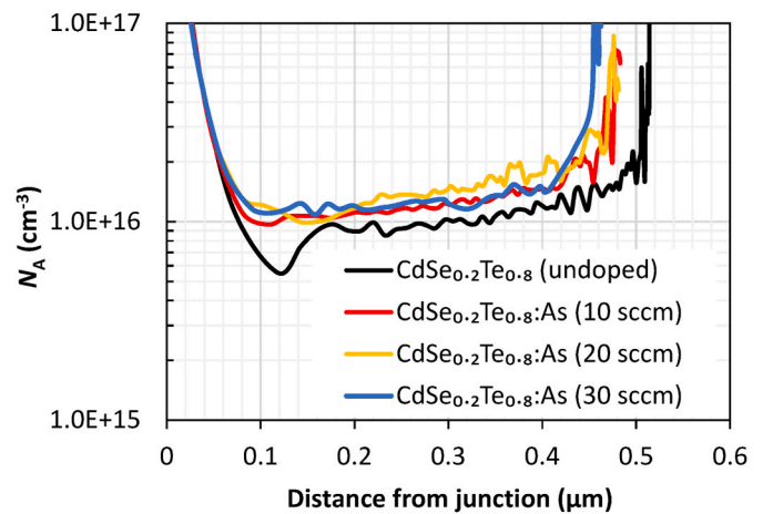
Fig. 11. Carrier concentration ( N_A ) of FTO/SnO 2 /CdSe/CdSe 0.2 Te 0.8 /CdTe:As devices with undoped and As doped Cd(Se, Te).
