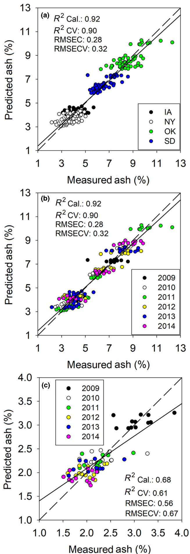
FIGURE 4 Measured ash versus ash predicted using environmental and production variables for upland switchgrass cultivars by location (a) and year (b) and for a lowland switchgrass cultivar by year (c). Solid line is the regression and the dashed line is the line of equality (slope=1, intercept=0)
