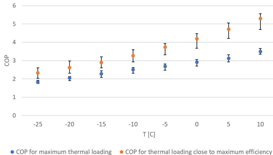
Steady-state COP vs. Temperature for All Heat Pump Models Combined
