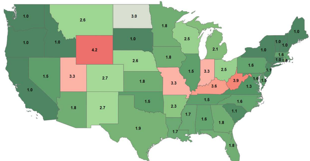
Minimum heat pump COP required for CO 2 e neutrality in each US state, compared with an 80 AFUE natural gas furnace.
