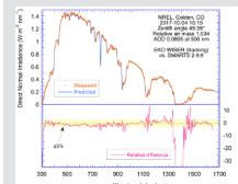
ASTM G173 vs. Measured Spectral Data
