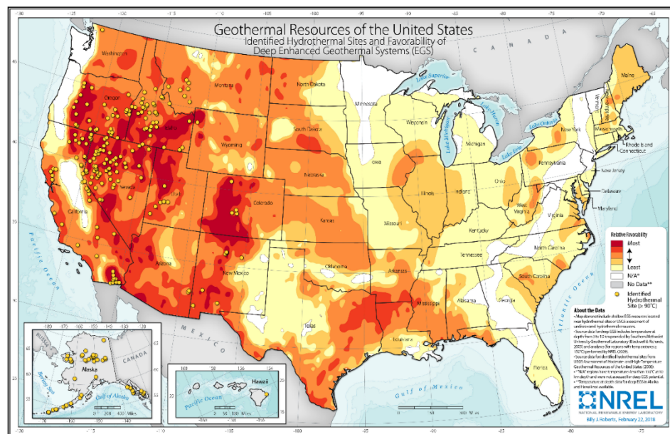
Figure 1: Deep EGS resource favorability and identified hydrothermal sites. Figure by Billy Roberts, NREL.
