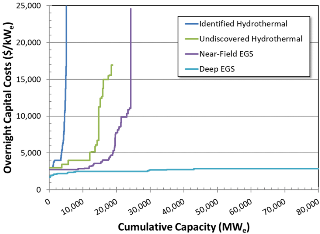
Figure 7: Extended view of available geothermal capacity (MW e ) at its modeled overnight capital cost ($/kW) by geothermal technology in 2030
