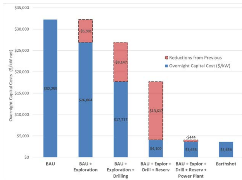
Figure 2: Cost reductions for the implementation of each parameter group seen in Table 1; BAU = business as usual
