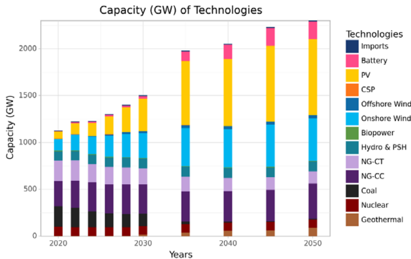
Figure 8: ReEDS model results for installed capacity by technology for the Enhanced Geothermal Shot analysis; CSP = concentrating solar power; PSH = pumped storage hydropower; NG = natural gas; CT = combustion turbine; CC = combined cycle
