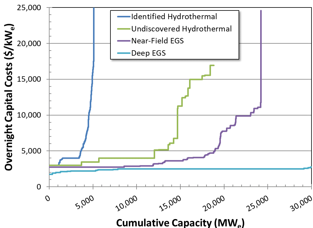
Figure 6: Available geothermal capacity (MW e ) at its modeled overnight capital cost ($/kW) by geothermal technology in 2030
