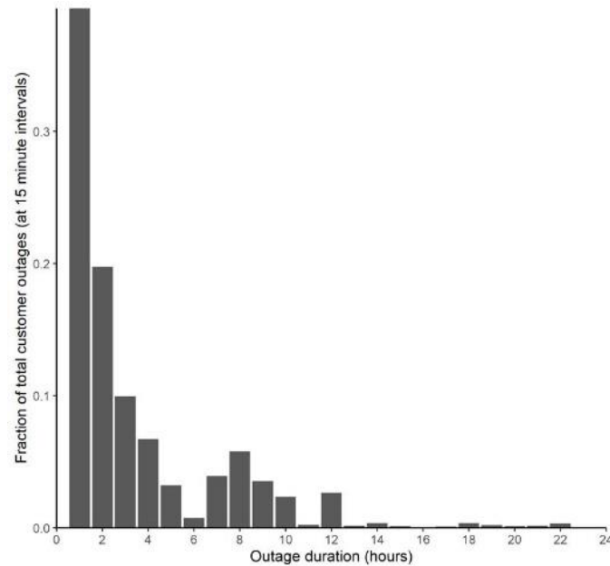
Figure 1. Customer outage and duration distribution probability function.
