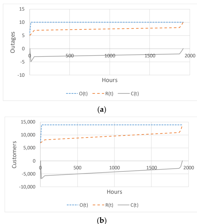
Figure 2. Component outage, restoration, and resilience curves for the hurricanes, (a) outage count and (b) unserved customers.
