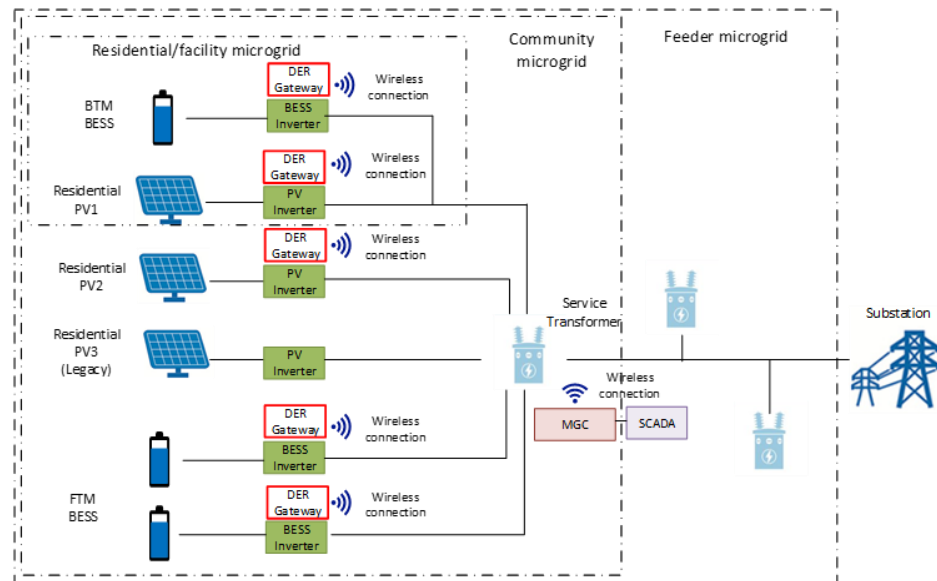
Figure 6. Resilient community microgrid layered approach using BTM and FTM DER assets as sublayer of diesel microgrid.
