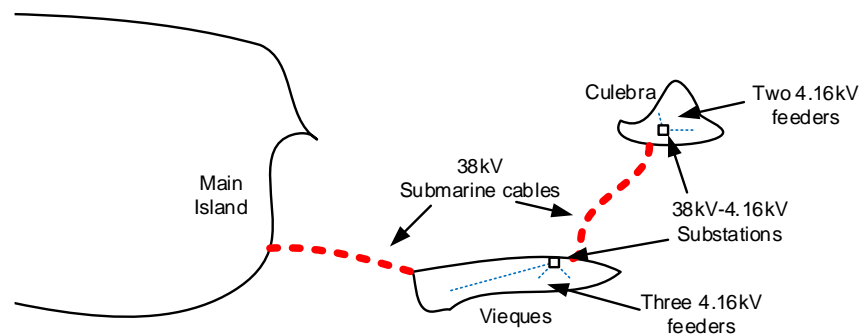
Figure 3. A simplified representation of the island system (not to scale).
