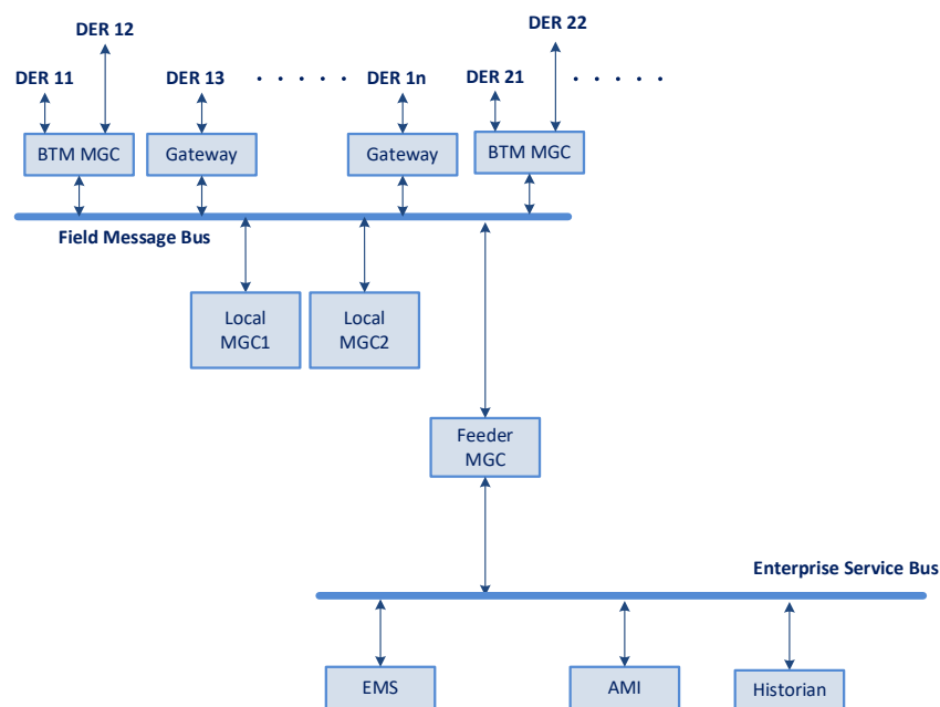
Figure 7. Resilient architecture for monitoring and control for the microgrids on both islands.
