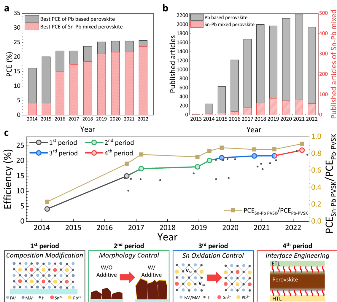
Fig. 1 Comparison of efficiency and research progress between Pb-based and Sn–Pb mixed based perovskite solar cells (PSCs). a Comparison of best efficiency by year of Pb-based and Sn–Pb mixed PSCs. b Number of publications by year of Pb-based and Sn–Pb mixed PSCs. c The reported efficiencies (left axis) of Sn–Pb mixed PSCs (dots on a graph). The larger, colorful dots above the line represent the highest efficiencies in each period and are important findings that distinguish research trends. The relative efficiency degree between Pb-based and Sn–Pb mixed PSCs (right axis). The schematic diagrams below show representative variables for each corresponding period of the research trend [15–40]
