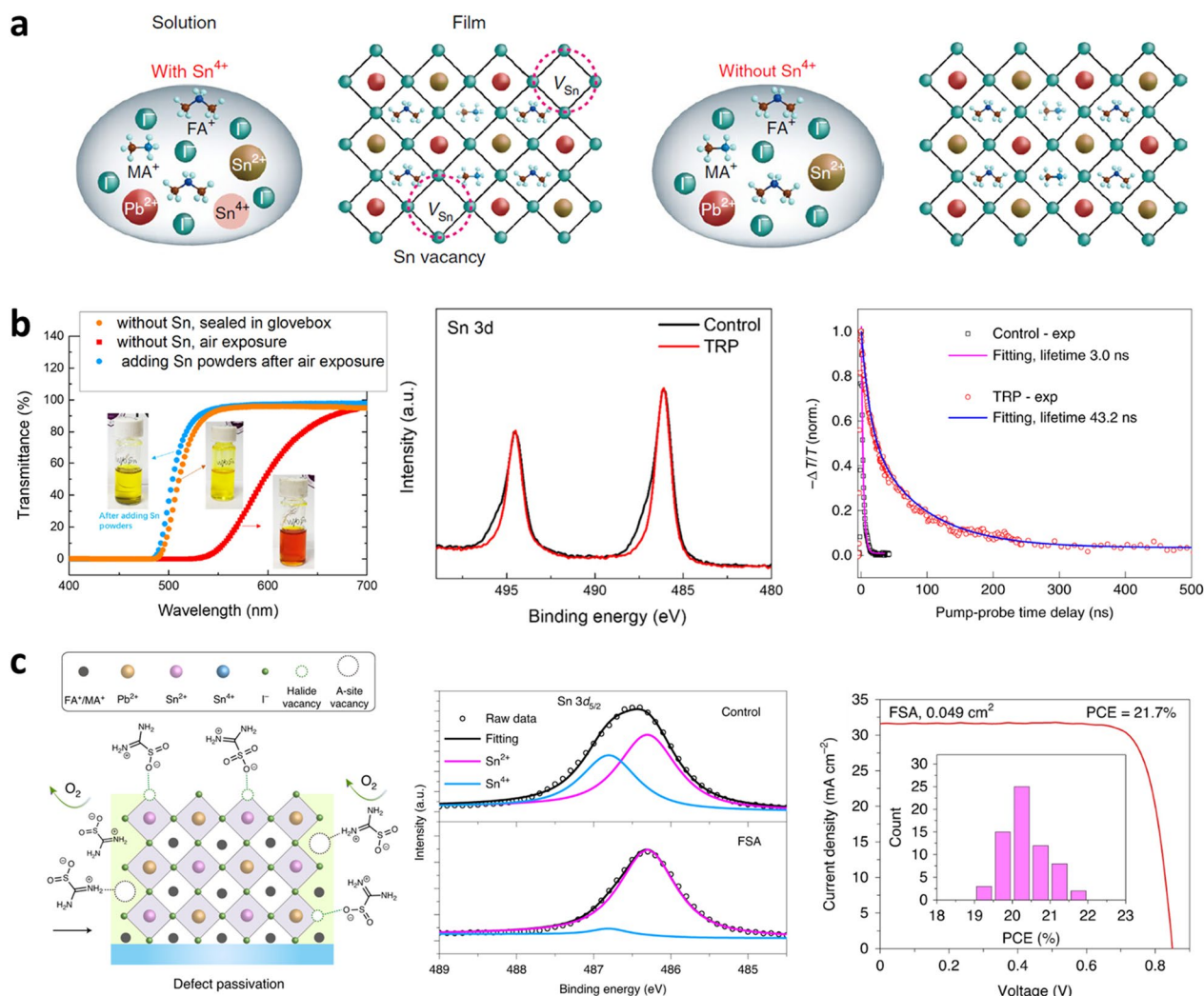
Fig. 6 Effect of reducing agents in precursor on Sn–Pb mixed perovskites. a Illustration of solution and crystal structure of Sn–Pb-based perovskite with and without reductant. b Transmittance, XPS, and TRPL decay without and with Sn metallic powder. Reproduced with permission from [17], copyright Springer Nature, 2019. c Schematic diagram of antioxidant and defect passivation with zwitterion FSA. XPS without and with FSA and J–V curve of Sn–Pb mixed PSC with FSA. Reproduced with permission from [18], copyright Springer Nature, 2020
