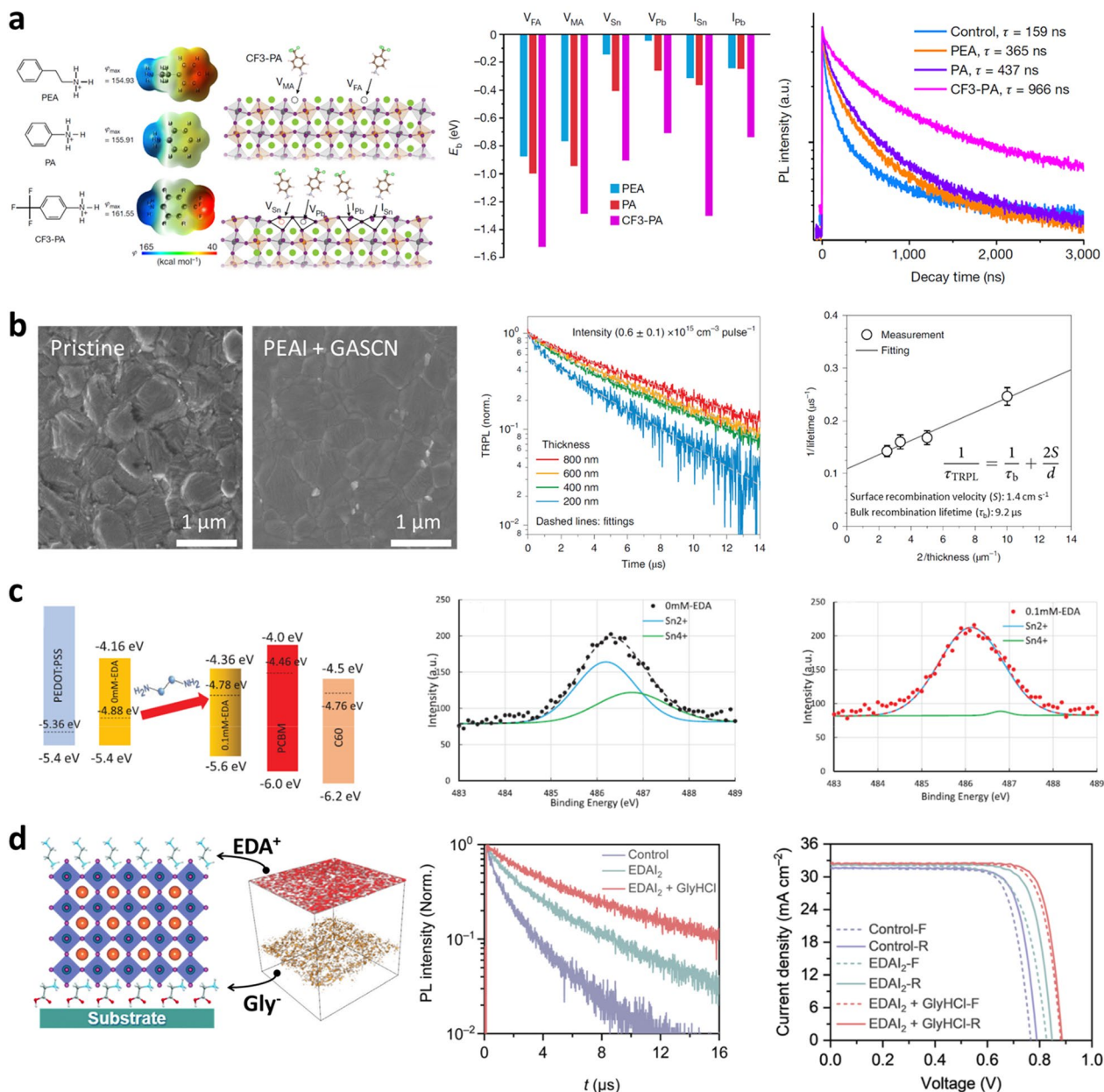
Fig. 7 Interface engineering of Sn–Pb mixed perovskites. a Schematic diagram of the interaction between ammonium cations and defects. The calculated binding energies of different passivators with various defects. TRPL decays of perovskite with different passivators. Reproduced with permission from [57], copyright Springer Nature, 2022. b SEM images of perovskite films without and with mixed PEA1 and GASCN additives. Thickness dependence of the TRPL measurements with mixed additives. Surface recombination velocity and bulk recombination lifetime plotted through carrier lifetime with various thickness. Reproduced with permission from [44], copyright Springer Nature, 2022. c XPS analysis of perovskite film with and without EDA treatment and energy diagram of PSC with and without EDA treatment. Reproduced with permission from [38], copyright John Wiley and Sons, 2021. d Schematic diagram of EDA 2+ and GlyH + cations forming dipoles at the perovskite interfaces. TRPL decay and J - V curves without and with surface treatments. Reproduced with permission from [40], copyright Royal Society of Chemistry, 2022
