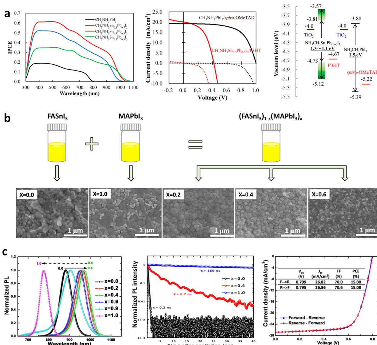
Fig. 4 Compositional and crystal structural improvement of Sn–Pb mixed perovskite for solar cells. a IPCE curves for MASn x Pb (1-x) I 3 PSCs and optimized photovoltaic performance for MASn 0.5 Pb 0.5 I 3 and MAPbI 3 PSCs. Energy diagram of MASn x Pb (1-x) I 3 perovskite. Reproduced with permission from [20], copyright American Chemical Society, 2014. b Schematic view of formation perovskite precursor and SEM images of (FASn 3 ) 1-x (MAPbI 3 ) x perovskite films. c Normalized PL spectra of (FASn 3 ) 1-x (MAPbI 3 ) x perovskites, TRPL of (FASn 3 ) 1-x (MAPbI 3 ) x perovskites at x=0.0, 0.4, 1.0 and J-V curves at x=0.4. Reproduced with permission from [15], copyright American Chemical Society, 2016
