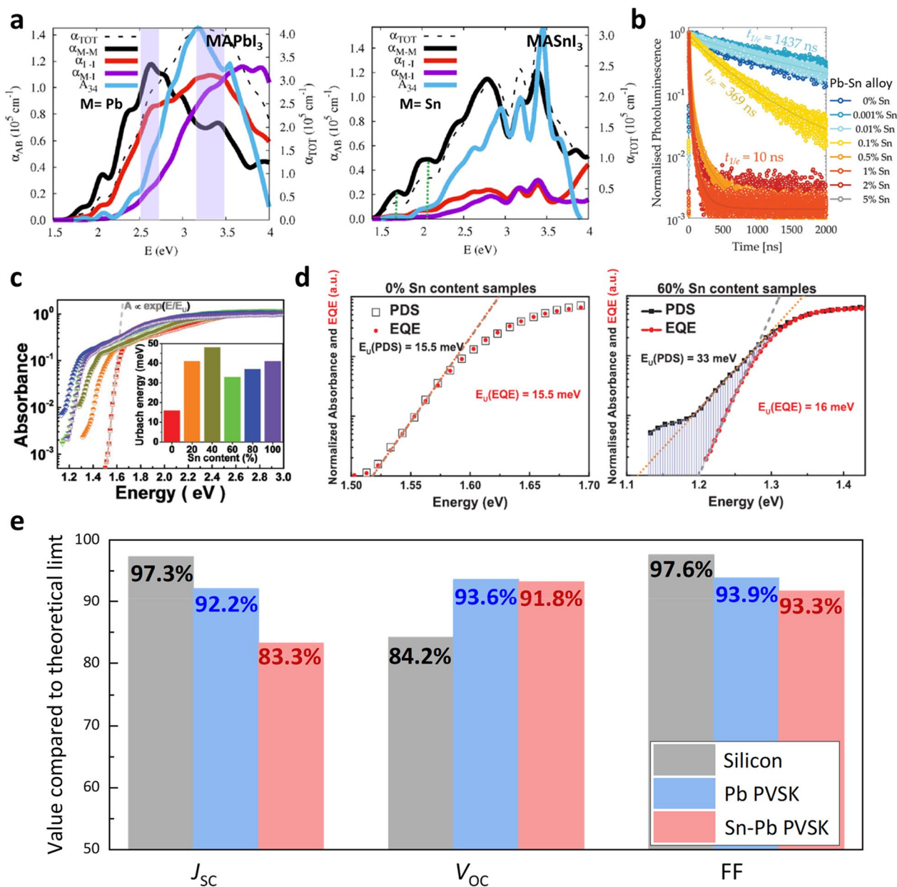
Fig. 3 Materials characteristics of Sn–Pb mixed perovskite and their status in terms of photovoltaic properties. a Absorption coefficient of \text{MAPbI}_3 and \text{MASnI}_3 . Reproduced with permission from [14], copyright American Chemical Society, 2018. b PL lifetime for different Sn concentrations in (\text{FA}_{0.83}\text{Cs}_{0.17})(\text{Pb}_{1-x}\text{Sn}_x)\text{I}_3 materials. Reproduced with permission from [49], copyright Royal Society of Chemistry, 2020. c Photothermal deflection spectroscopy (PDS) spectra of \text{MASn}_{1-x}\text{Pb}_x\text{I}_3 perovskite film with varying Sn concentration. d Normalized PDS and EQE spectra of \text{MASn}_{1-x}\text{Pb}_x\text{I}_3 perovskite. Reproduced with permission from [50], copyright John Wiley and Sons, 2016. e Comparison of each parameter of the current highest efficiency silicon, Pb-based and Sn–Pb mixed solar cells as a percentage compared to the theoretical efficiency SQ-limit [10, 40, 51]
