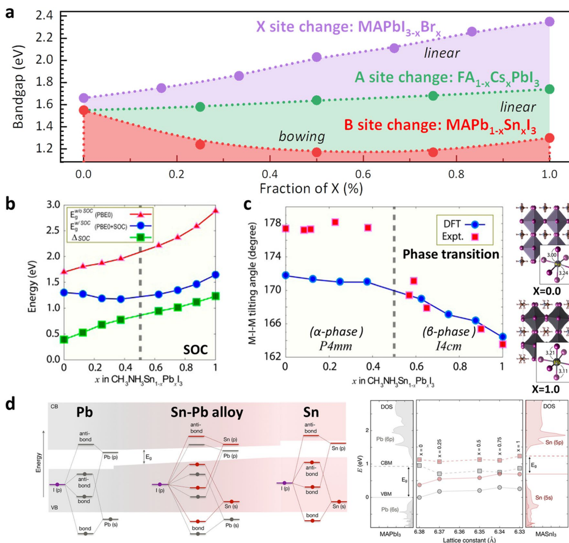
Fig. 2 Bandgap structure of Sn–Pb mixed perovskite. a The bandgap according to each site change in \text{ABX}_3 perovskite composition [21, 45, 46]. b Bandgap trend of \text{MASn}_{1-x}\text{Pb}_x\text{I}_3 without SOC and with SOC, and the difference in bandgaps without SOC and with SOC, \Delta_{\text{SOC}} . Reproduced with permission from [47], copyright American Chemical Society, 2015. c M–I–M tilting angle as a function of x in \text{MASn}_{1-x}\text{Pb}_x\text{I}_3 . Crystal structures of x=0.0 and 1.0 . Reproduced with permission from [47], copyright American Chemical Society, 2015. d The bandgap bowing in \text{MA}(\text{Pb}_{1-x}\text{Sn}_x)\text{I}_3 and reduction in the bandgap of alloy compositions by the effect of strain on the band edge energies of pure compositions. Reproduced with permission from [48], copyright American Chemical Society, 2018
