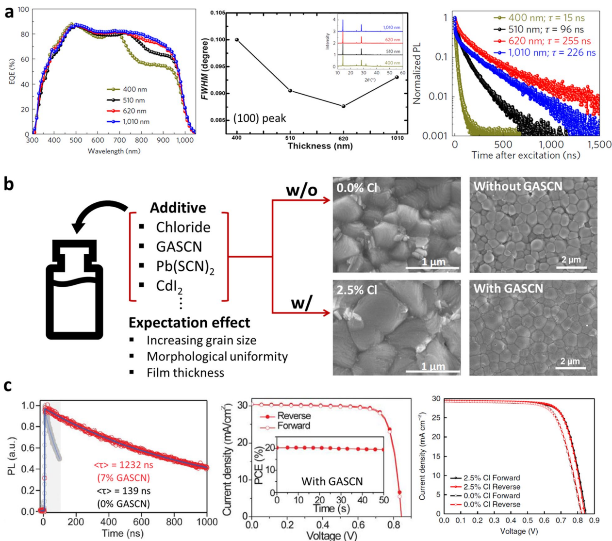
Fig. 5 Precursor design via concentration and additives for improving perovskite film quality. a EQE curves, XRD FWHM values of (100) peak and carrier lifetime via TRPL of (\text{FASnI}_3)_{1-x}(\text{MAPbI}_3)_x perovskite with different thickness. Reproduced with permission from [53], copyright Springer Nature, 2017. b Various additives effects on the morphological evolution of Sn–Pb perovskite confirmed by SEM. c Carrier lifetime via TRPL and J - V curves of perovskite solar cells and with and without additives. Reproduced with permission from [28], copyright The American Association for the Advancement of Science, 2019. Reproduced with permission from [16], copyright Springer Nature, 2018
