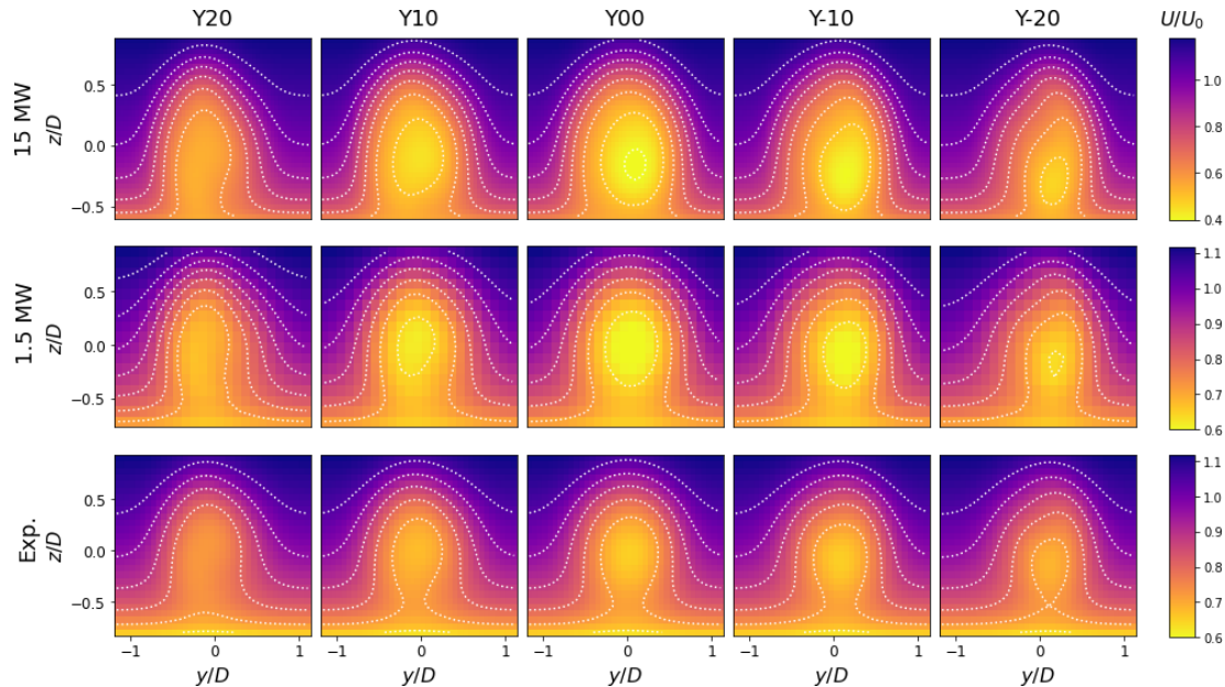
Figure 8. FLORIS streamwise flow fields across yaw angles at x/D = 3 for 15 MW (top panels), 1.5 MW (middle panels), and scaled model turbine (bottom panels) inputs. Wake deformation is visible for yawed cases since the curled wake model includes the counter-rotating vortex pair.
