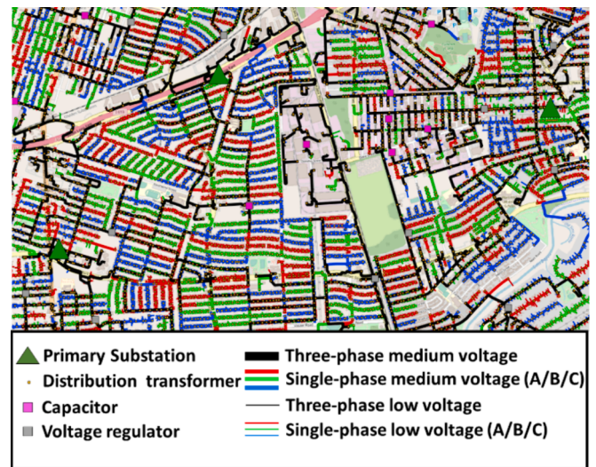
Fig. 7. Medium-voltage network.
