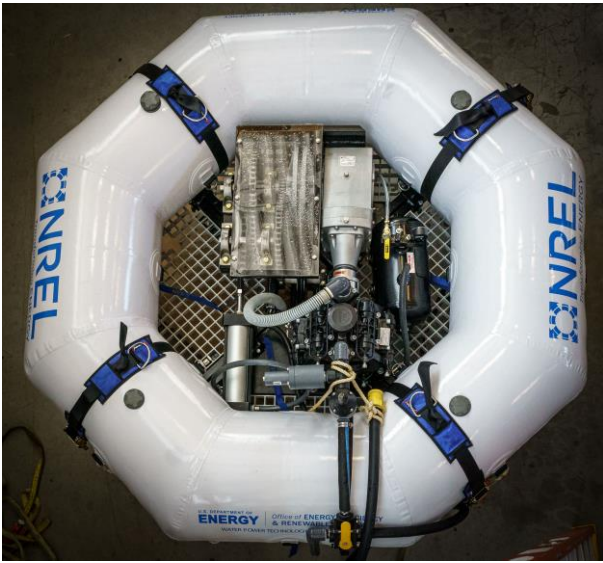
Fig. 1. A top-down view of the HERO WEC, in the hydraulic configuration, prior to its deployment at the test site in North Carolina, USA (image credit: Andrew Simms, NREL)
