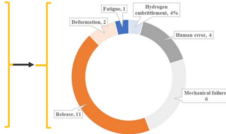
Breakdown of "external leak-hydrogen" events by failure mechanism
