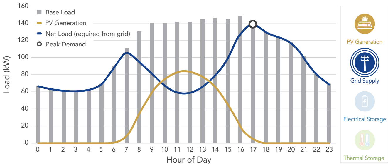
Figure 2. Graph showing on-site solar PV production during a sunny day and its effect on the net load required from grid. The relatively small level of PV generation offsets a portion of the building electrical loads, resulting in a reduced net load through the primary daylight hours.
