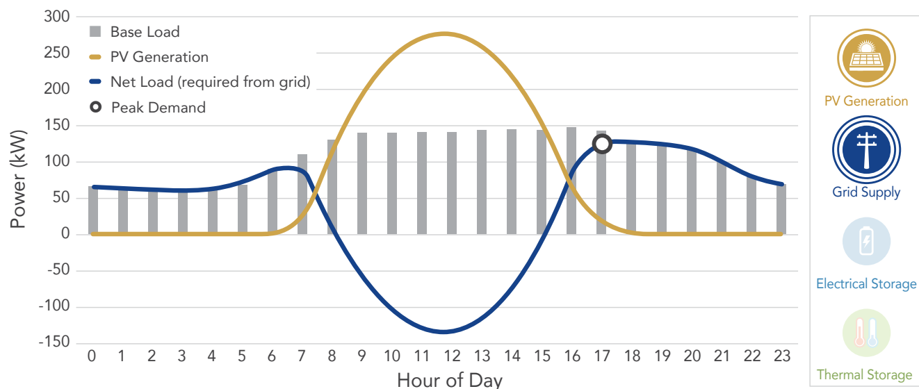
Figure 3. Graph showing production from a larger on-site solar PV array and its effect on the net load the facility requires from the grid. The presence of a negative net load indicates that there is more on-site generation than the facility can consume. In this case, the negative net load values represent excess generation that would need to either be exported to the grid or curtailed.
