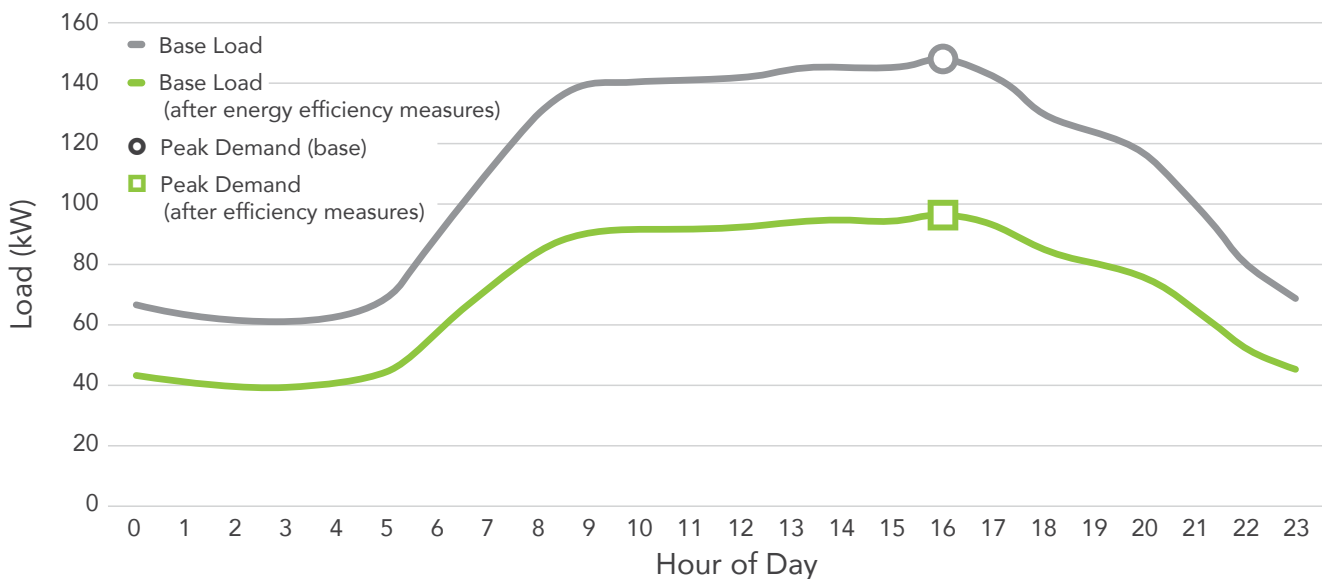
Figure 7. Graph showing the potential of energy efficiency strategies to reduce building energy consumption. Energy efficiency measures can yield large load reductions that can facilitate building electrification without the need for capacity increases. 19
