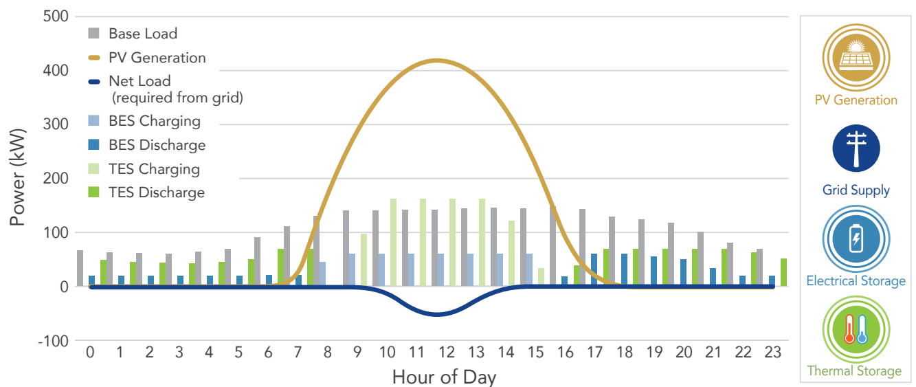
Figure 6. Graph showing the production from an even larger on-site solar PV array, the charge/discharge of both a BES and a larger TES system, and their effect on the net load. To further reduce the grid exports, the facility would need to curtail a fraction of the total on-site generation.
