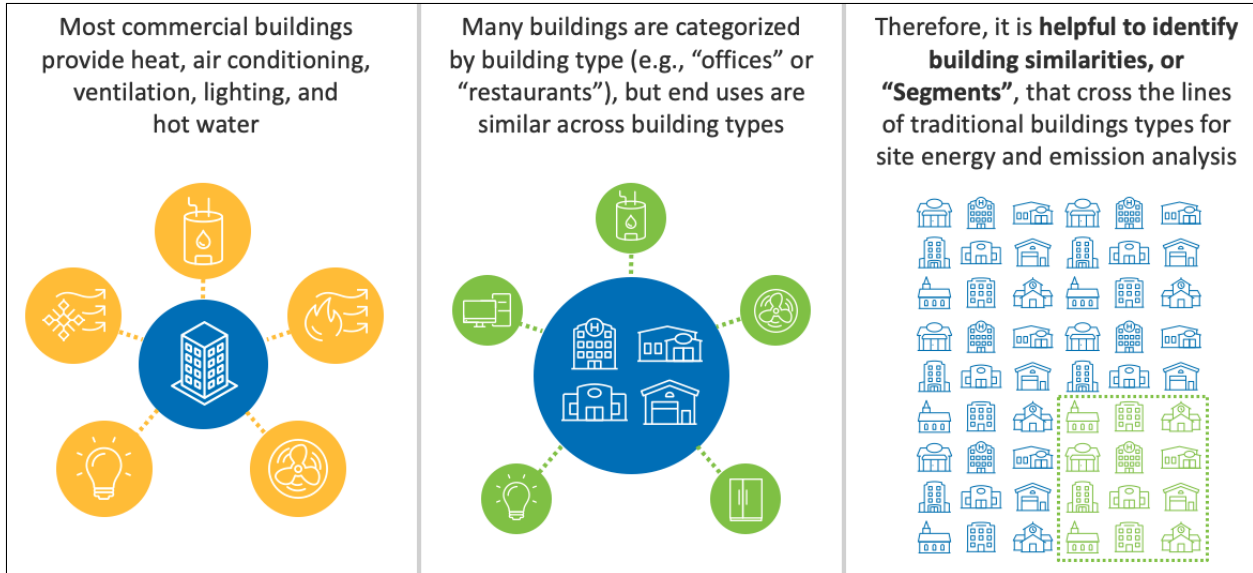
Figure 1. Segmentation Analysis
