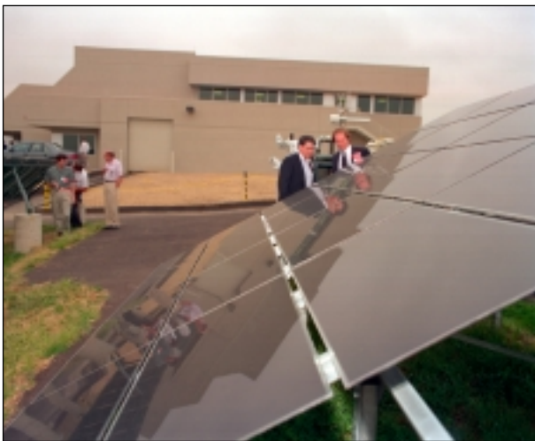
NREL field tests of a 1-kW Solar Cells, Inc., CdTe system show no output degradation over three years.
