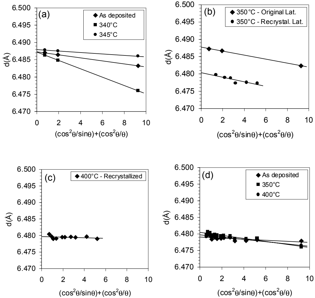
FIGURE 2. Lattice parameter of CSS CdTe thin films before and after CdCl 2 treatment. (a)(b)(c) LT films. (d) HT films.
