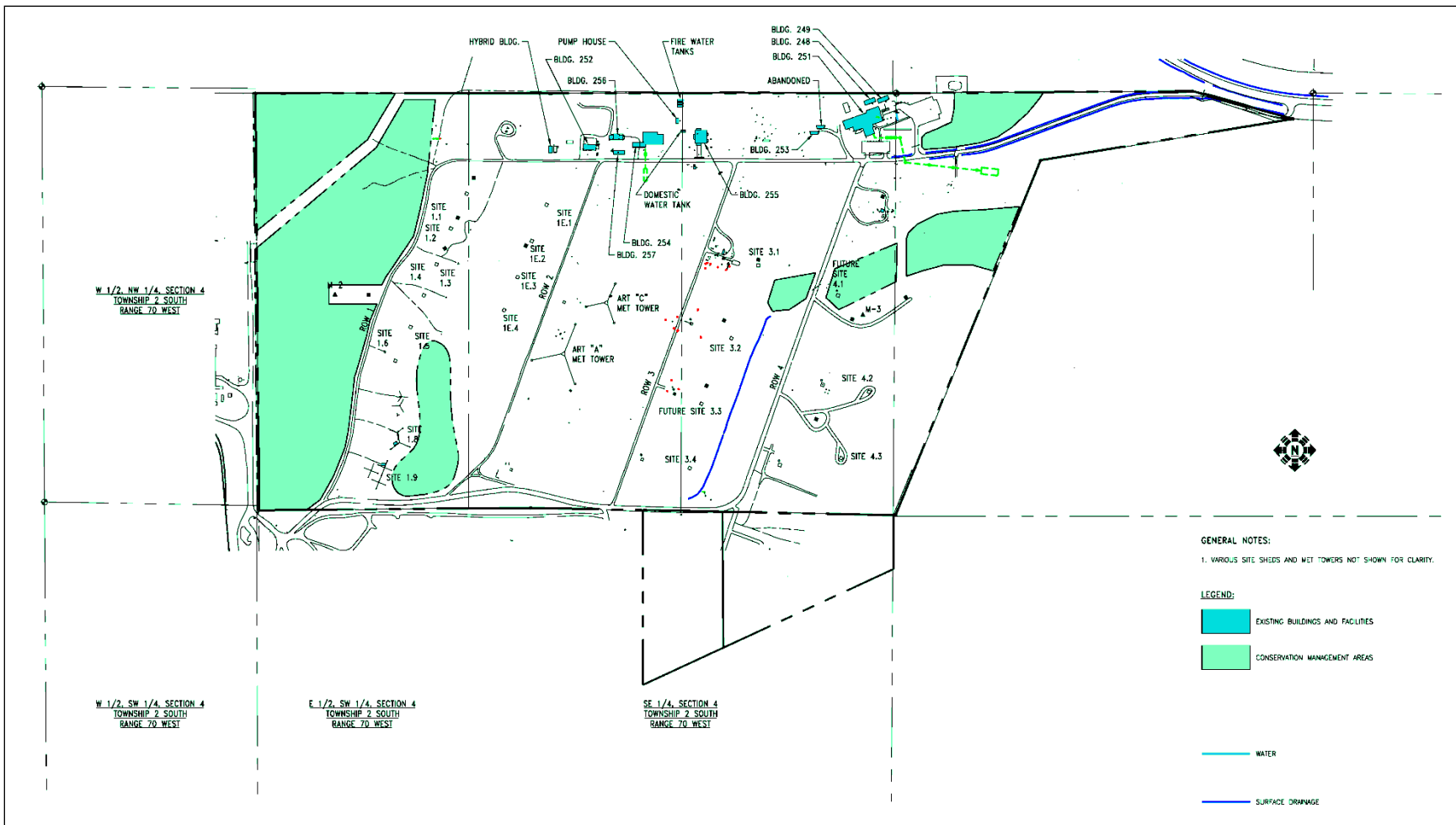
Figure 4. NWTC site detail
