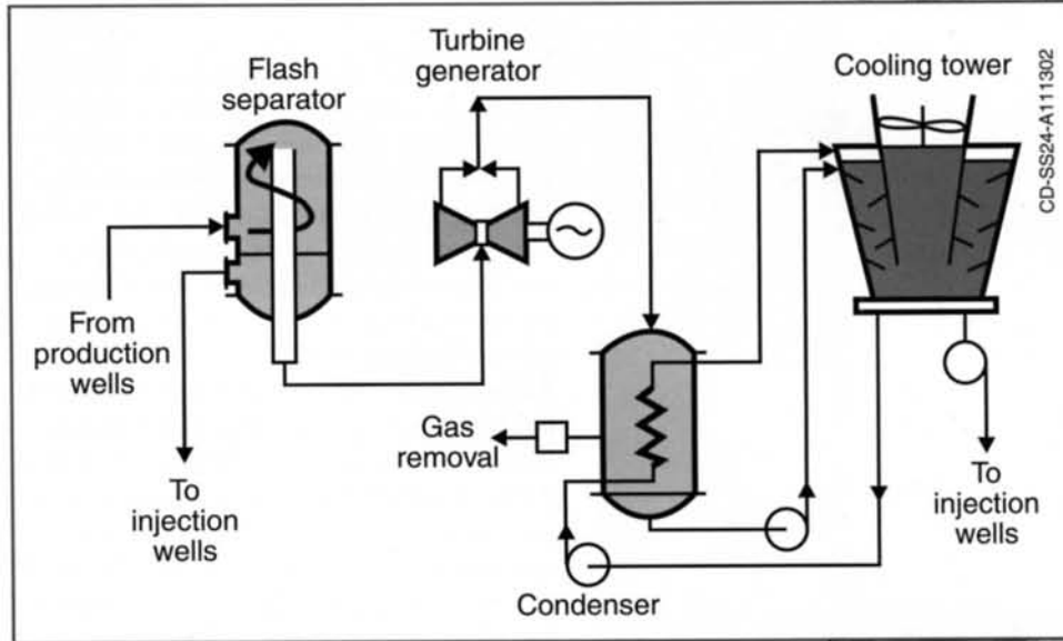
Flash-steam technology is used for high-temperature geothermal liquids. The geothermal liquid is flashed to steam, which drives a turbine.
