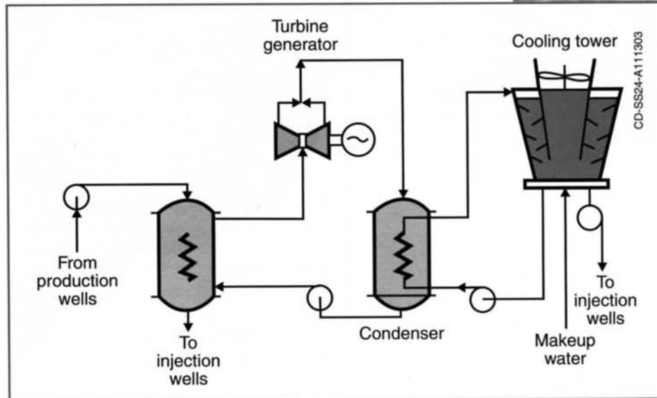
Binary cycle technology is used for moderate-temperature geothermal liquids. The geothermal liquid vaporizes a working fluid in the heat exchanger, and the working-fluid vapor drives a turbine.
