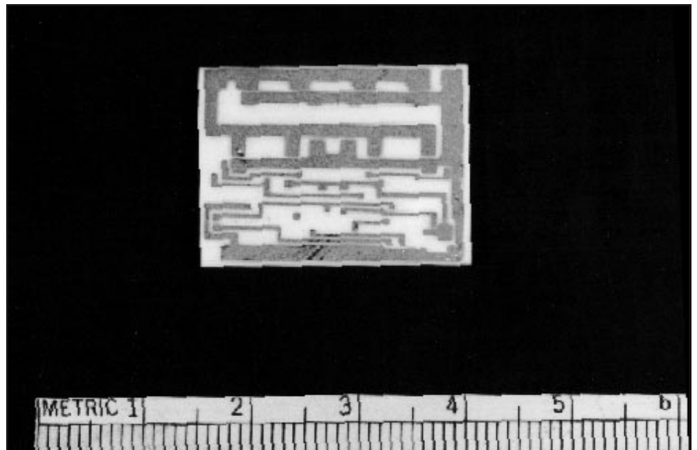
A metallized ceramic circuit—consisting of a thin copper film bonded to a beryllium oxide substrate—manufactured by Brush Wellman. The SI Program and Brush Wellman are experimenting with using high solar flux to produce these electronic components.
