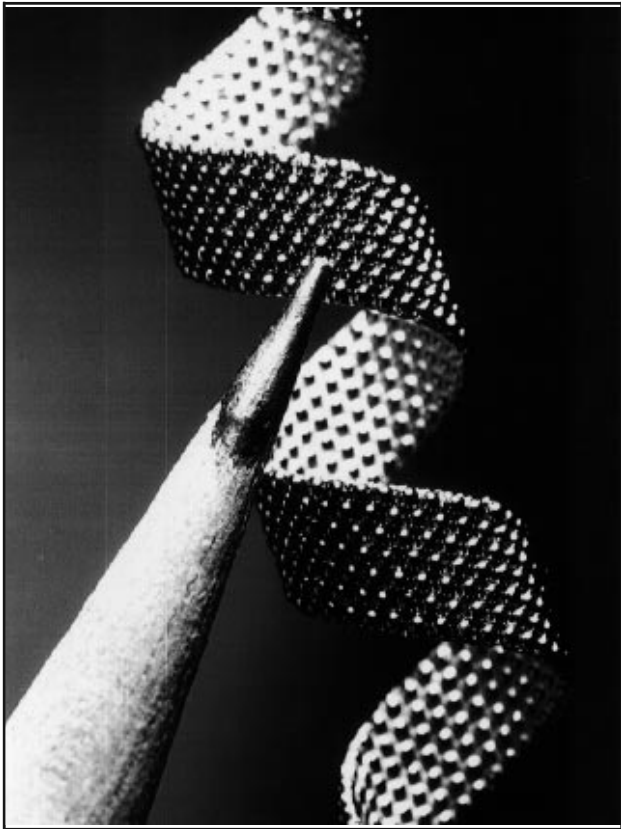
In 1994 Texas Instruments and the SI Program explored manufacturing spherical photovoltaic cells like these with solar energy.
