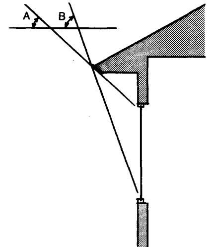
South Overhang Sizing In Birmingham, an ideally sized south overhang should allow full exposure of the window when the sun has a noon altitude of 37 degrees (angle A) and fully shade the window when the sun has a noon altitude of 74 degrees (angle B).
